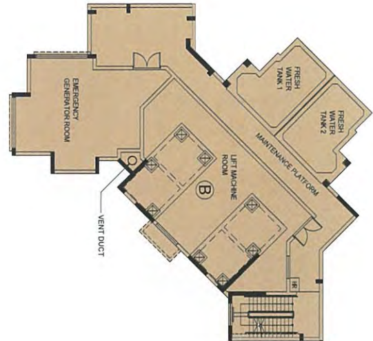
LIFT MACHINE ROOM PLAN
