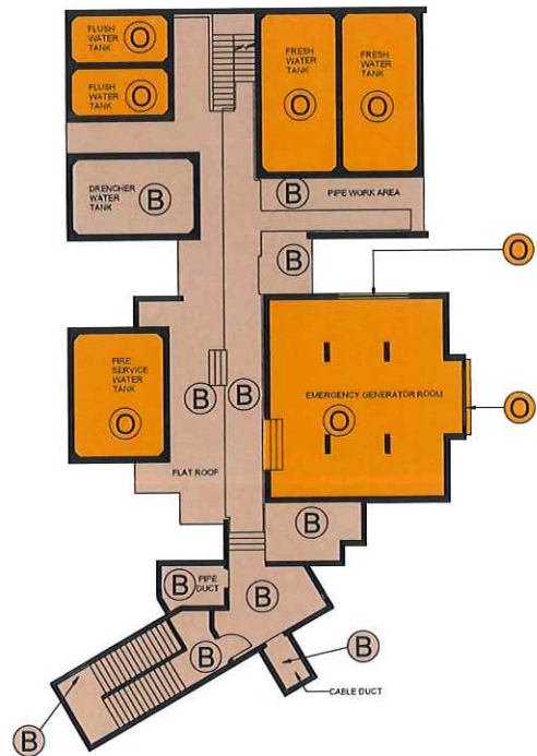
UPPER ROOF PLAN
