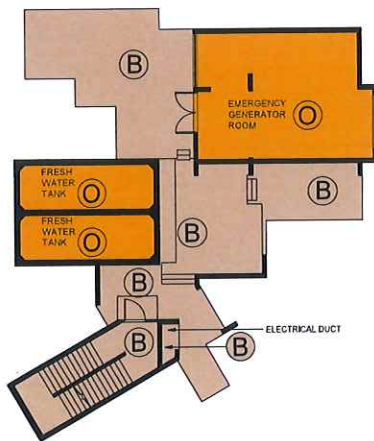
UPPER ROOF PLAN
