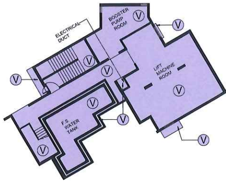
LIFT MACHINE ROOM FLOOR PLAN
