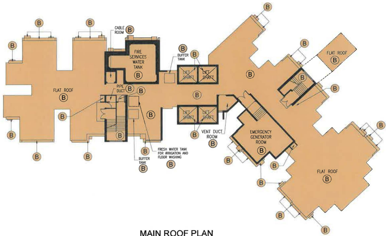
MAIN ROOF PLAN
