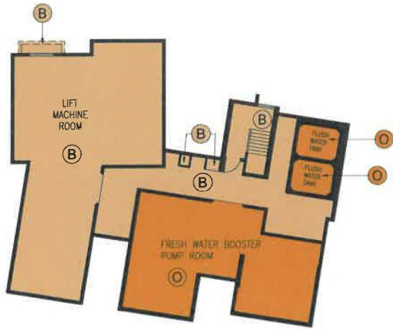
LIFT MACHINE ROOM PLAN
