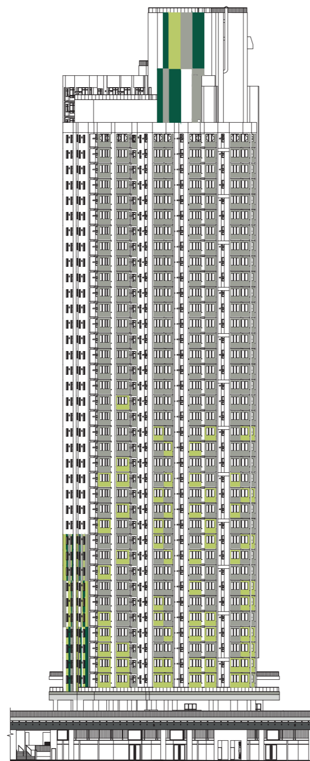
西南面立面圖“2” South West Elevation Plan "2"
