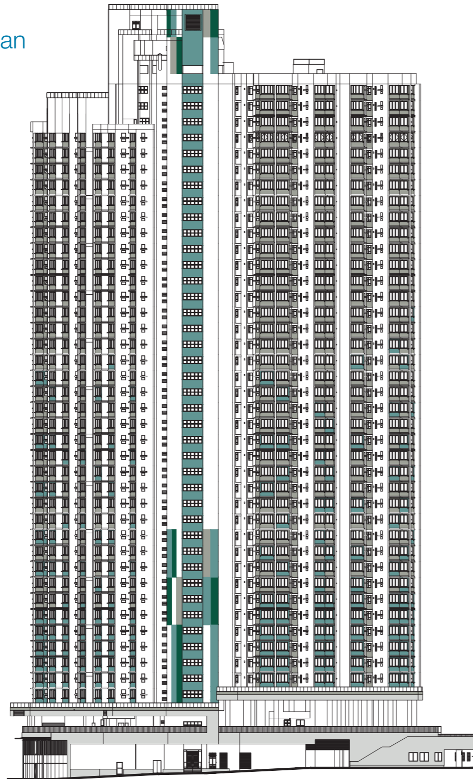
東南面立面圖“3” South East Elevation Plan “3”
