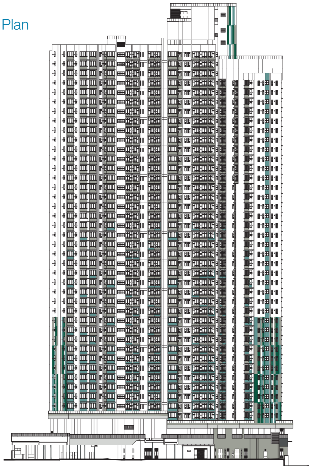
西北面立面圖“1” North West Elevation Plan “1”
