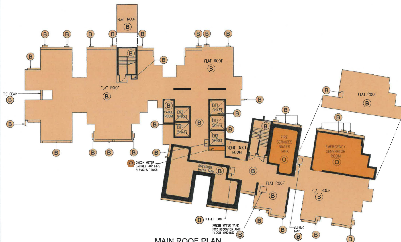
MAIN ROOF PLAN
