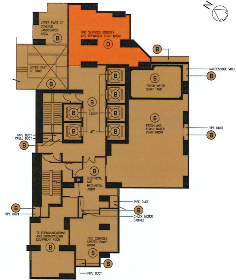
LOWER GROUND 1ST FLOOR (AT LEVEL +16.30)
