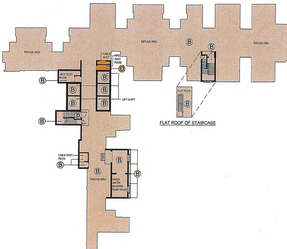
MAIN ROOF PLAN
