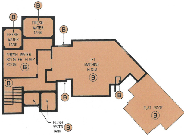
LIFT MACHINE ROOM PLAN
