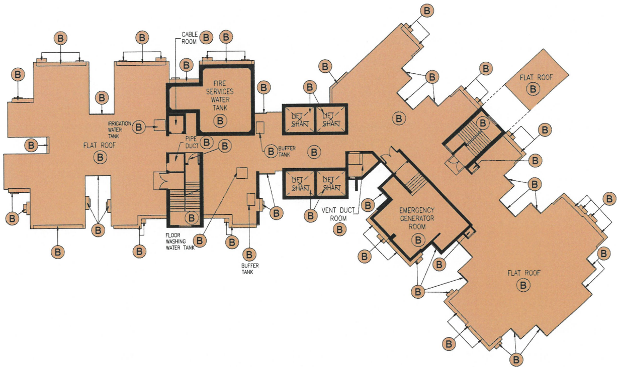
MAIN ROOF PLAN
