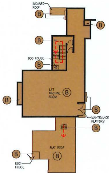
UPPER ROOF PLAN AT LEVEL +124.75
