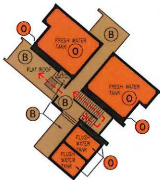
UPPER ROOF PLAN AT LEVEL +124.95
