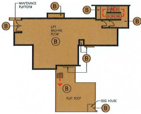
UPPER ROOF PLAN AT LEVEL +124.75
