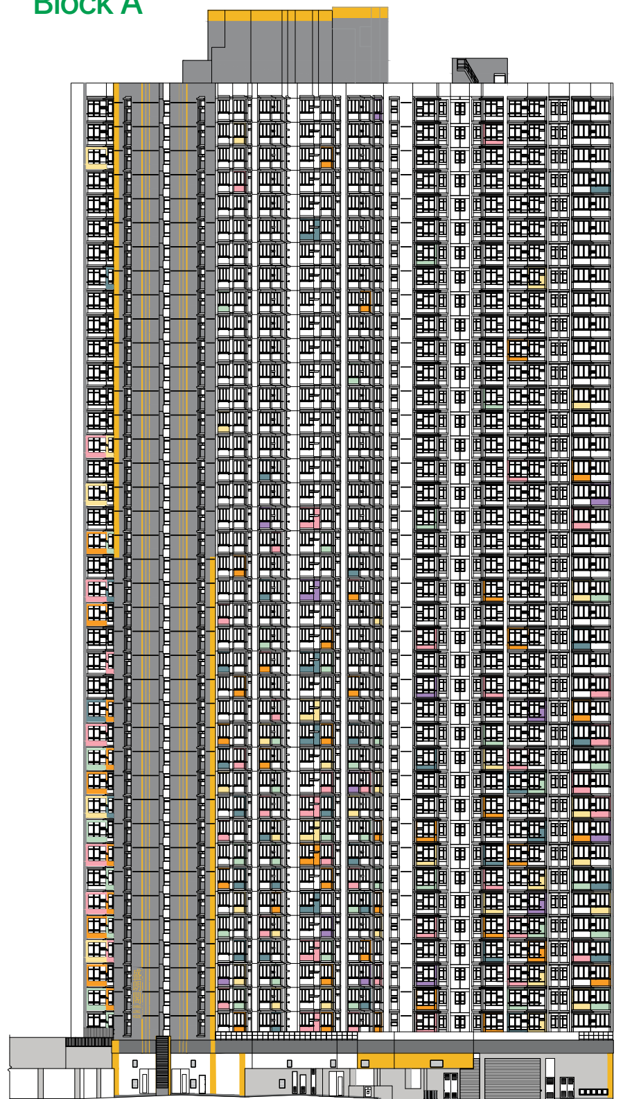
南面立面圖 "1" South Elevation Plan "1"
