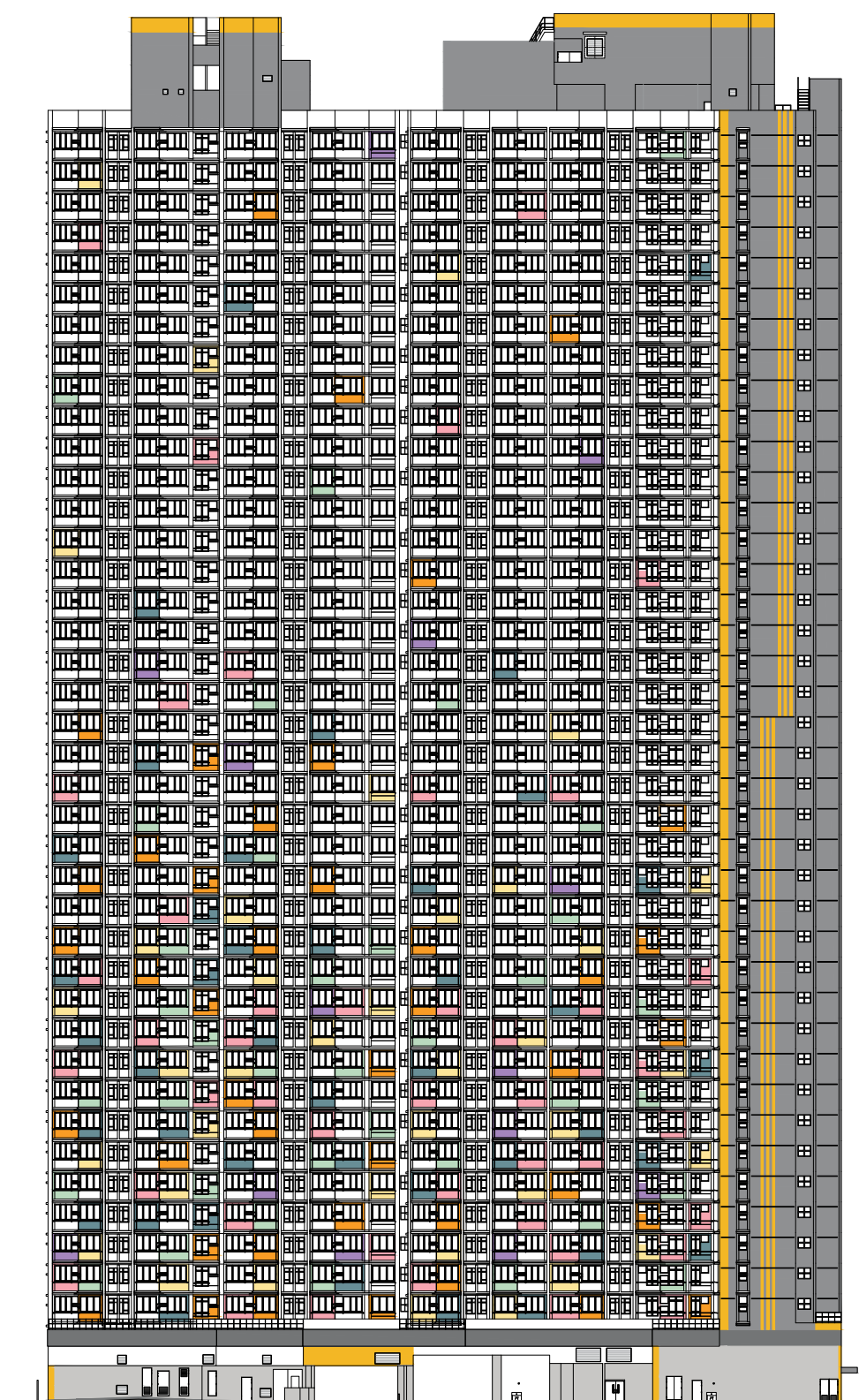
東面立面圖 "2" East Elevation Plan "2"
