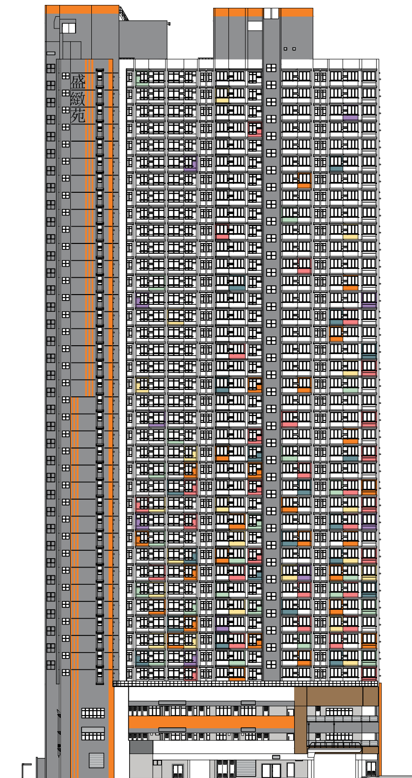
西南面立面圖 "8" South West Elevation Plan "8"
