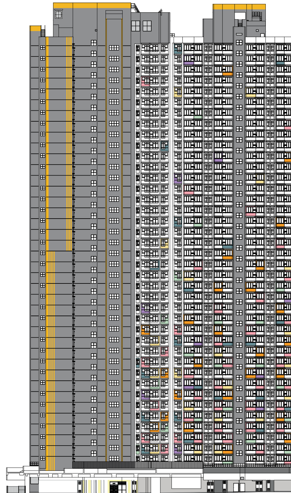
西面立面圖"4" West Elevation Plan "4"
