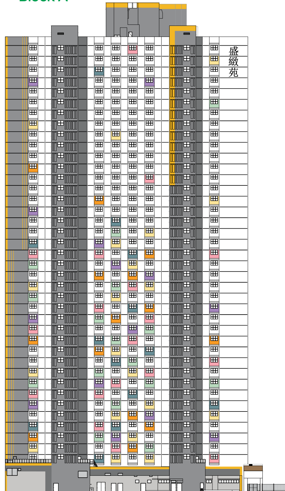
北面立面圖"3" North Elevation Plan "3"
