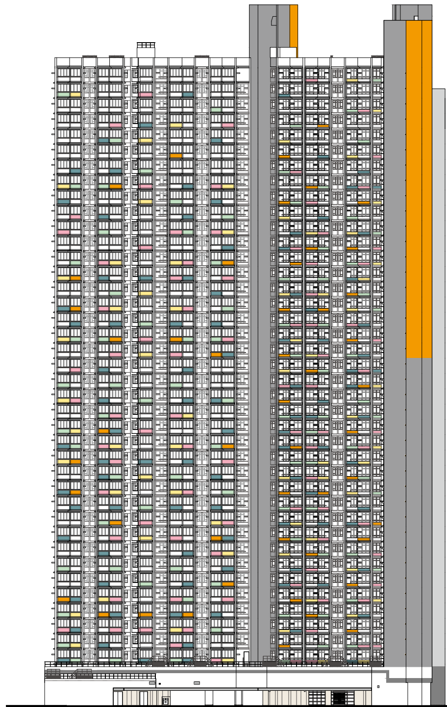
東面立面圖 "1" East Elevation Plan "1"
