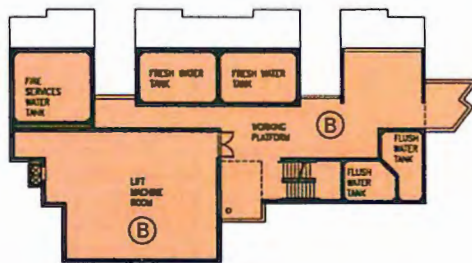
LIFT MACHINE ROOM PLAN
