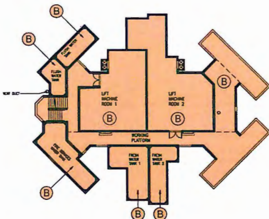
LIFT MACHINE ROOM PLAN
