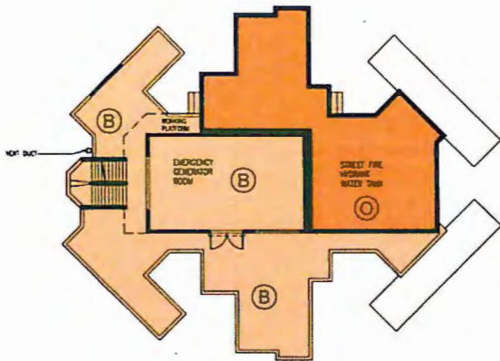
EMERGENCY GENERATOR ROOM PLAN
