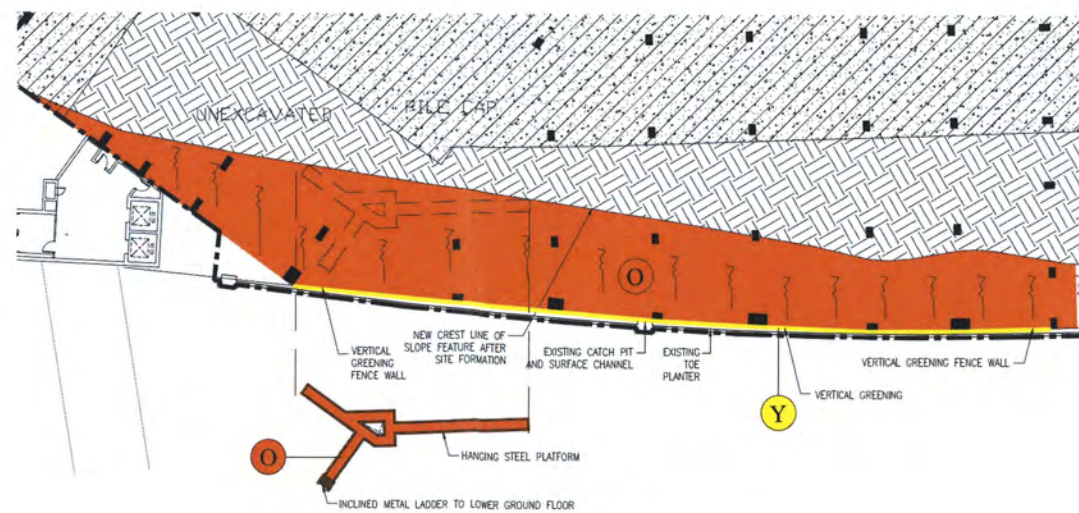
PART PLAN OF HANGING STEEL PLATFORM
