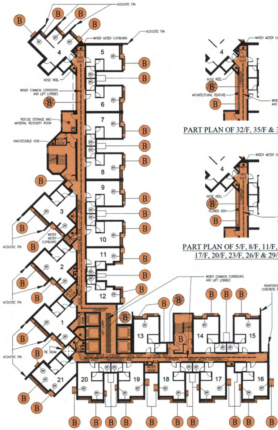
PART PLAN OF 14/F
