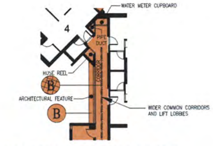
PART PLAN OF 32/F, 35/F & 38/F
