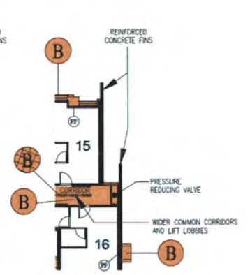
PART PLAN OF 14/F
