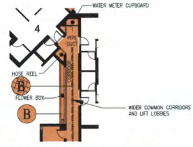
PART PLAN OF 5/F, 8/F, 11/F, 14/F, 17/F, 20/F, 23/F, 26/F & 29/F
