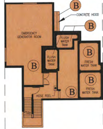
UPPER ROOF 2 PLAN
