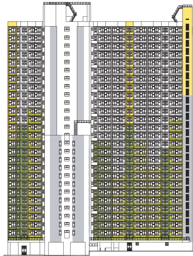
東面立面圖“4” East Elevation Plan “4”
