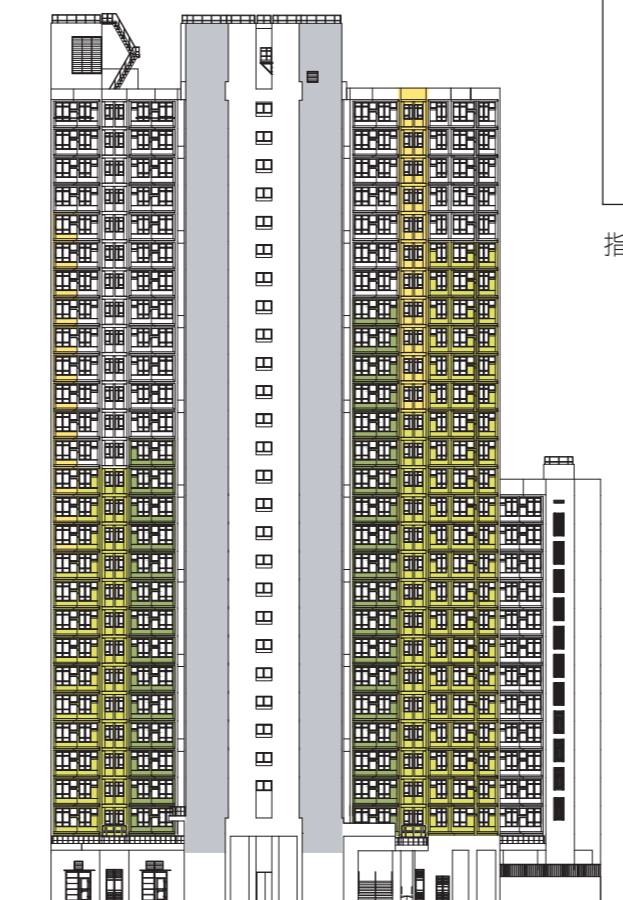
西北面立面圖“2” North West Elevation Plan “2”
