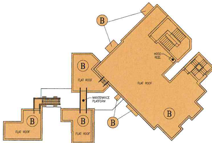
TOP ROOF PLAN
