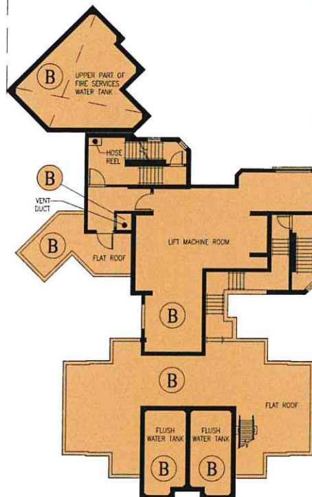
UPPER ROOF PLAN
