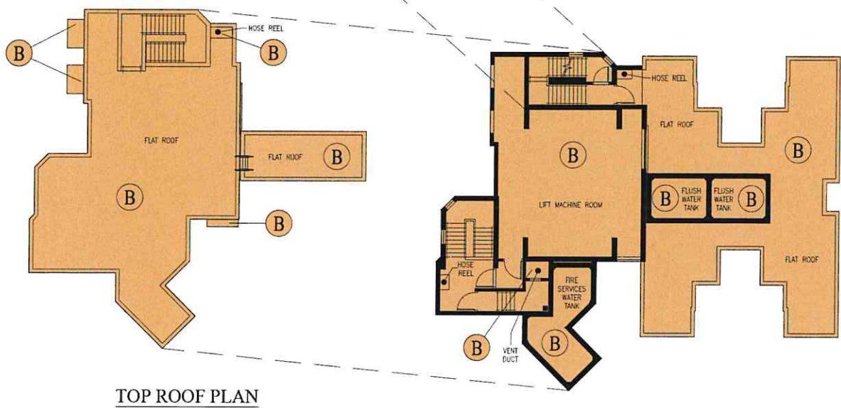
UPPER ROOF 1 PLAN
