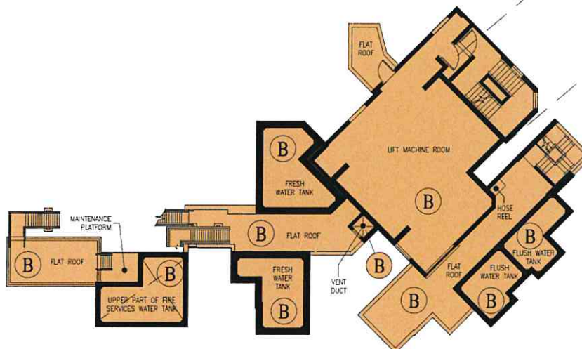
UPPER ROOF 1 PLAN
