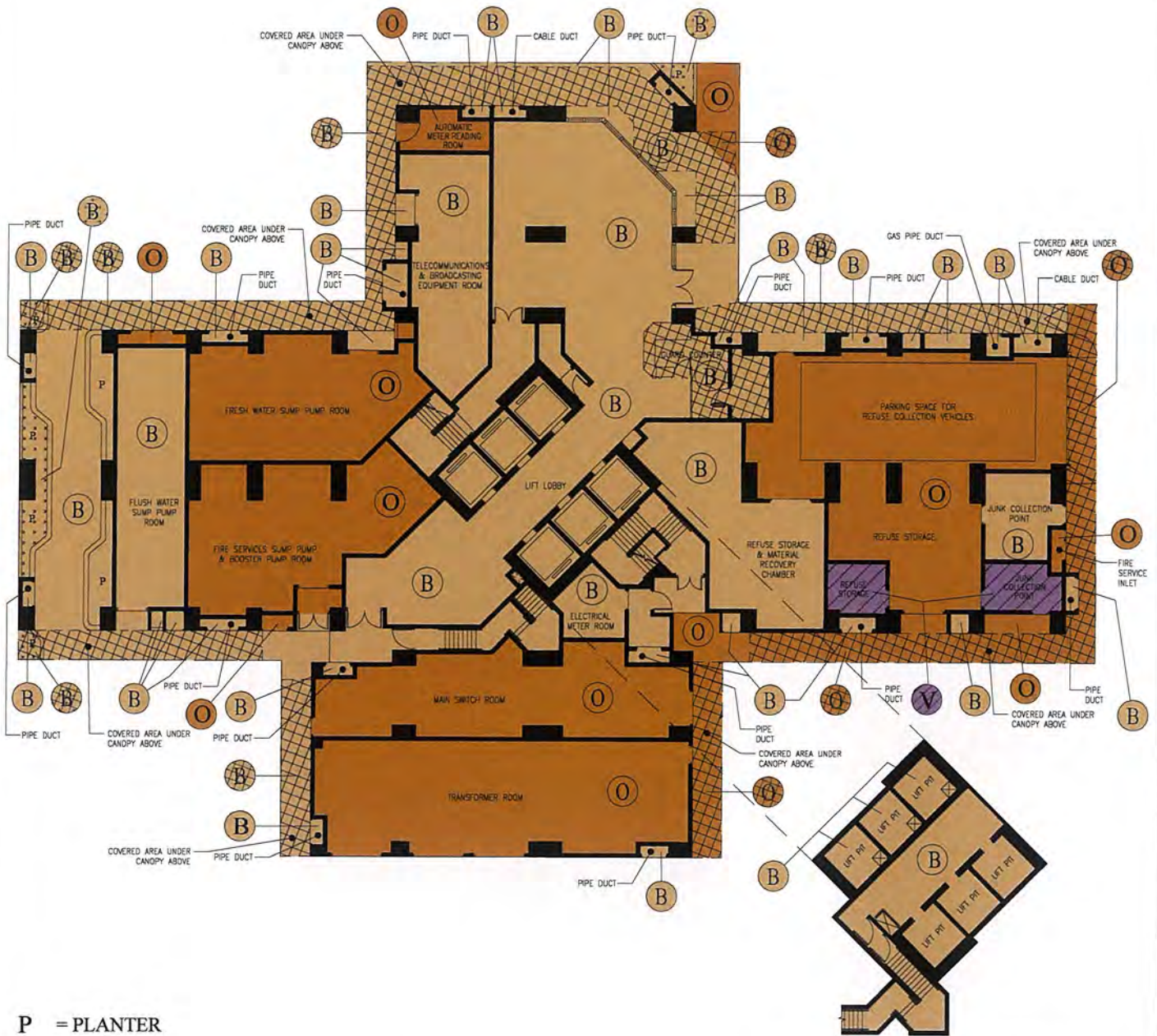
PART PLAN OF LIFT PITS BELOW
