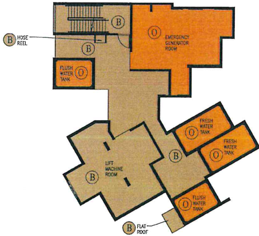
LIFT MACHINE ROOM PLAN
