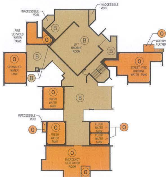
UPPER ROOF PLAN
