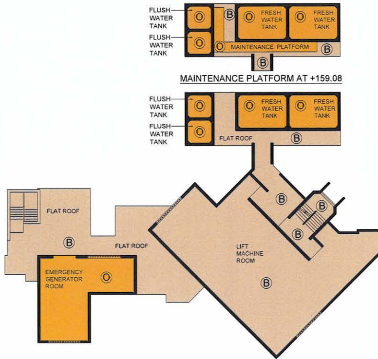
LIFT MACHINE ROOM PLAN
