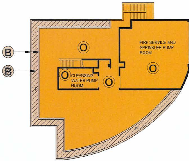
MAIN ROOF PLAN
