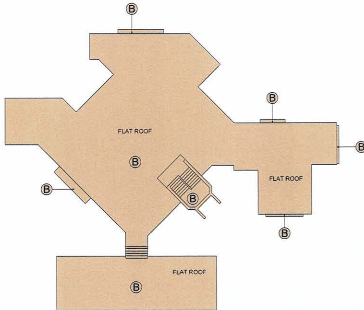
TOP ROOF PLAN
