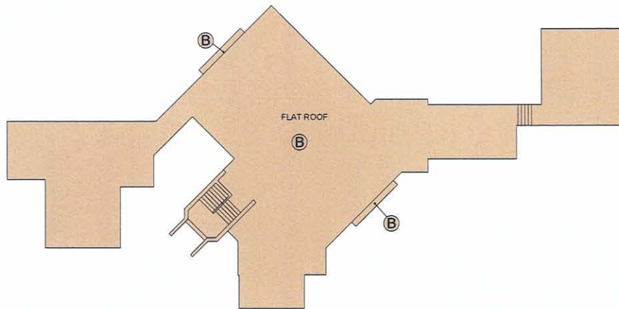
TOP ROOF PLAN
