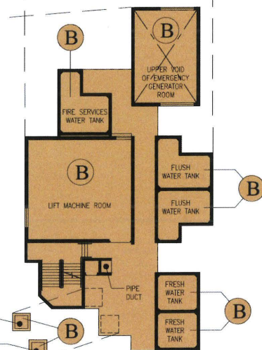
LIFT MACHINE ROOM PLAN
