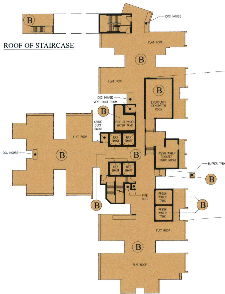
MAIN ROOF PLAN
