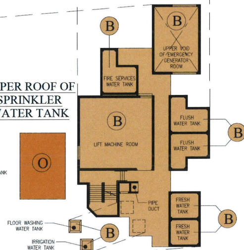
LIFT MACHINE ROOM PLAN
