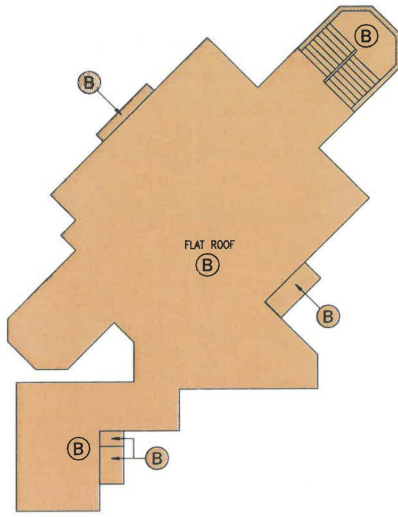
TOP ROOF PLAN
