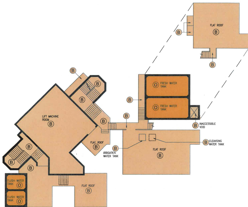
LIFT MACHINE ROOM FLOOR PLAN
