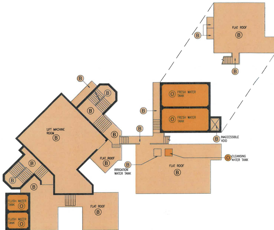
LIFT MACHINE ROOM FLOOR PLAN
