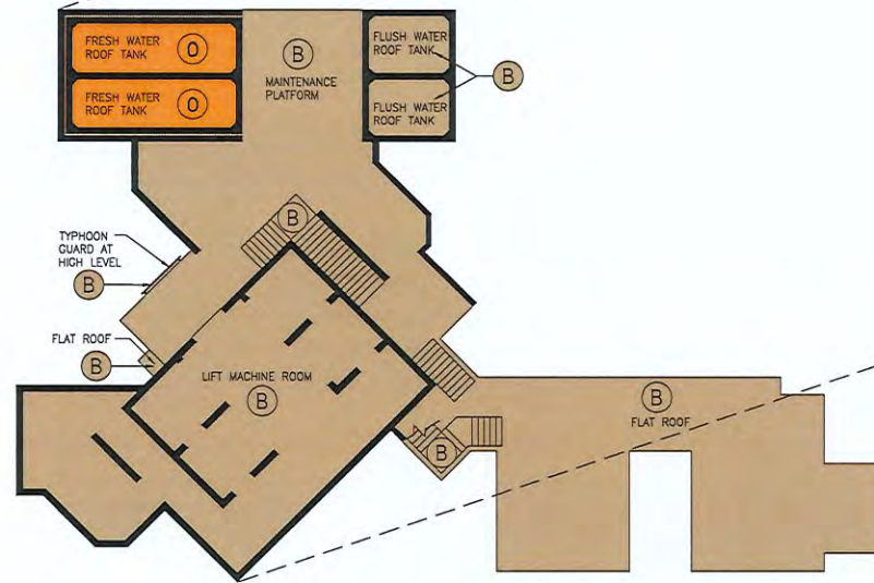
LIFT MACHINE ROOM FLOOR PLAN
