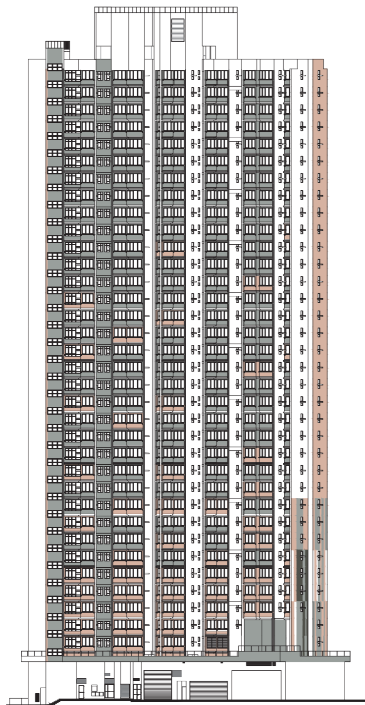
東面立面圖“1” East Elevation Plan “1”
