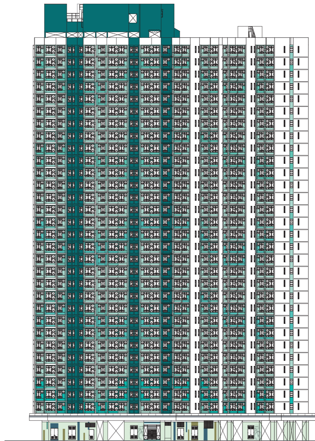
北面立面圖“2” North Elevation Plan “2”
