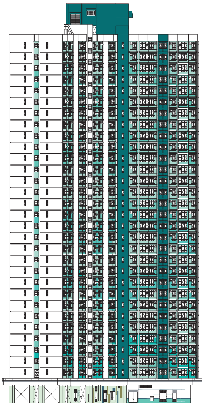
西面立面圖“3” West Elevation Plan “3”
