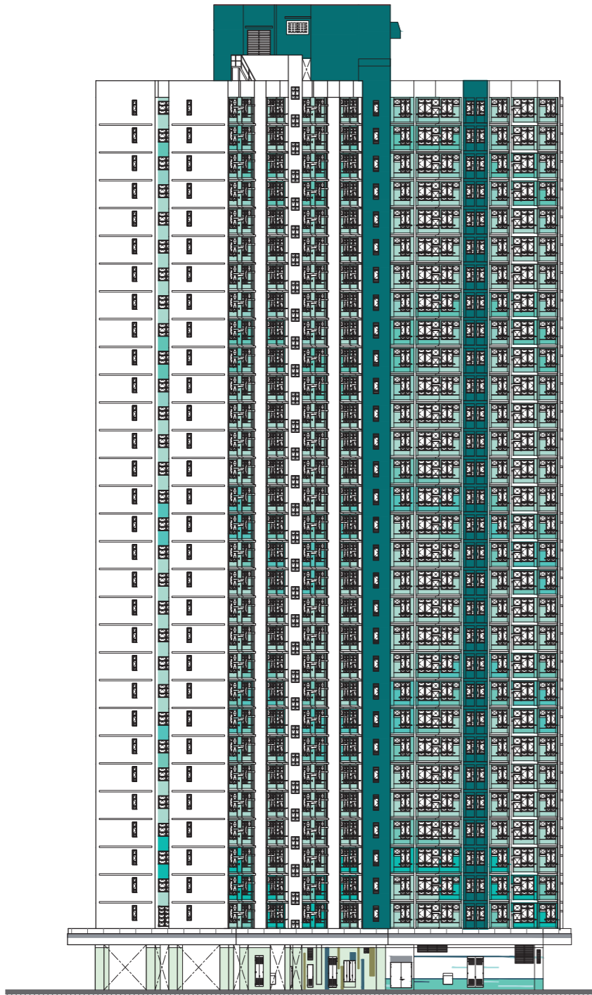
西南面立面圖“3” South West Elevation Plan “3”
