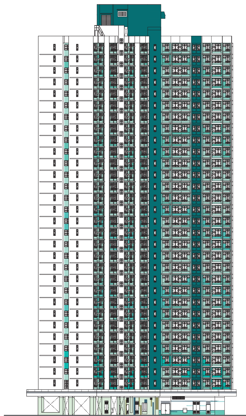
西面立面圖“3” West Elevation Plan “3”
