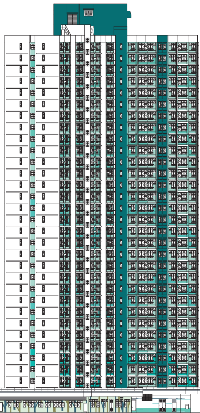
西南面立面圖“3” South West Elevation Plan “3”
