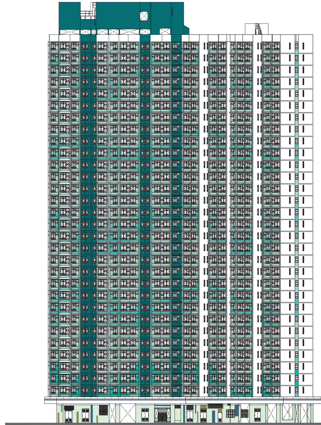
北面立面圖“2” North Elevation Plan “2”
