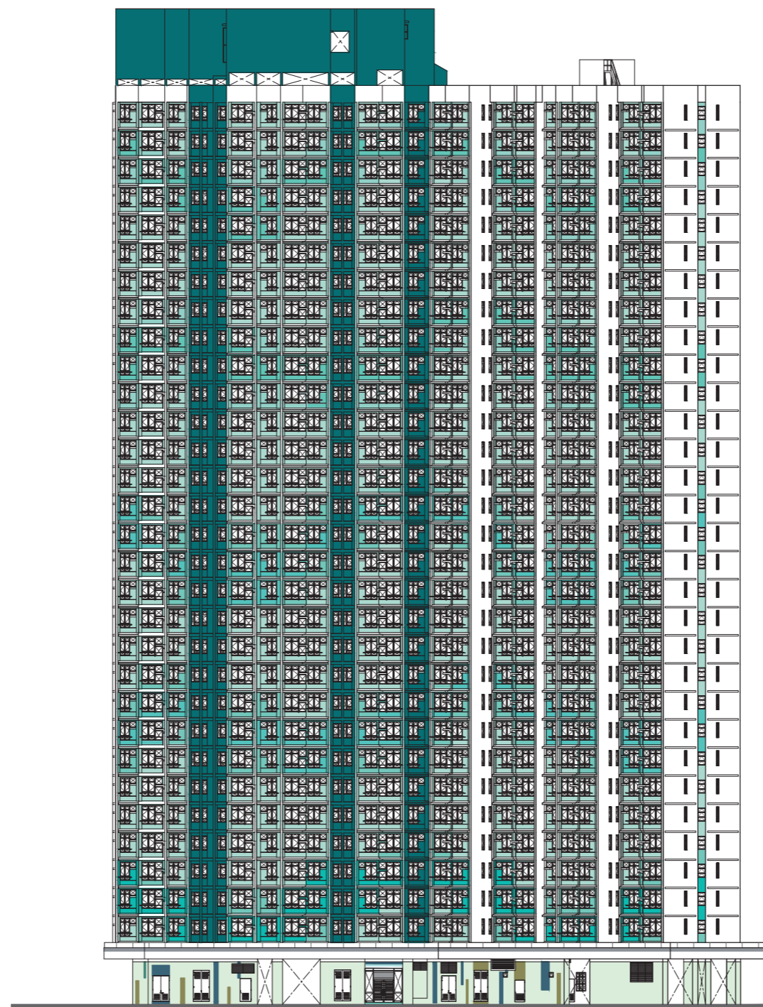
西北面立面圖“2” North West Elevation Plan “2”
