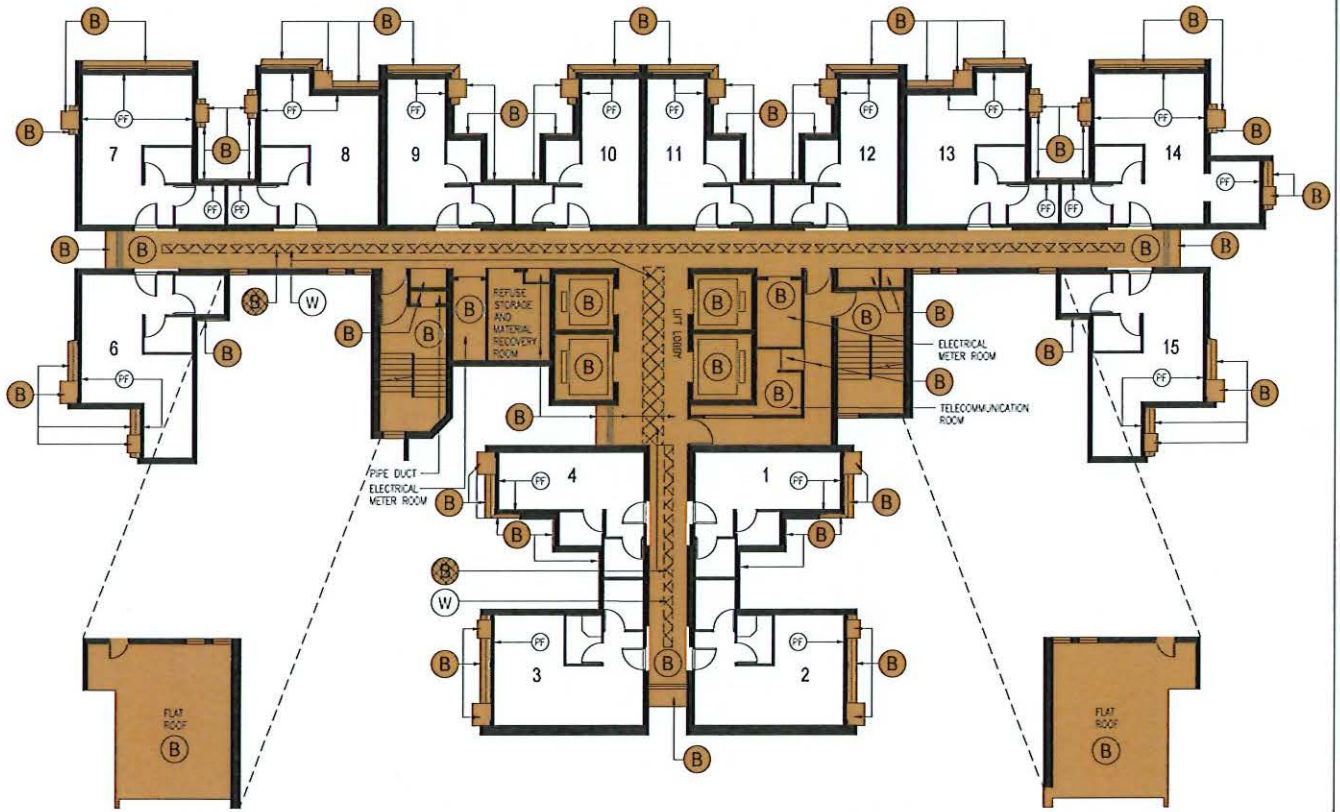
PART PLAN AT 35/F ONLY
