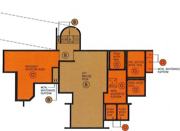
UPPER ROOF FIRST FLOOR PLAN
