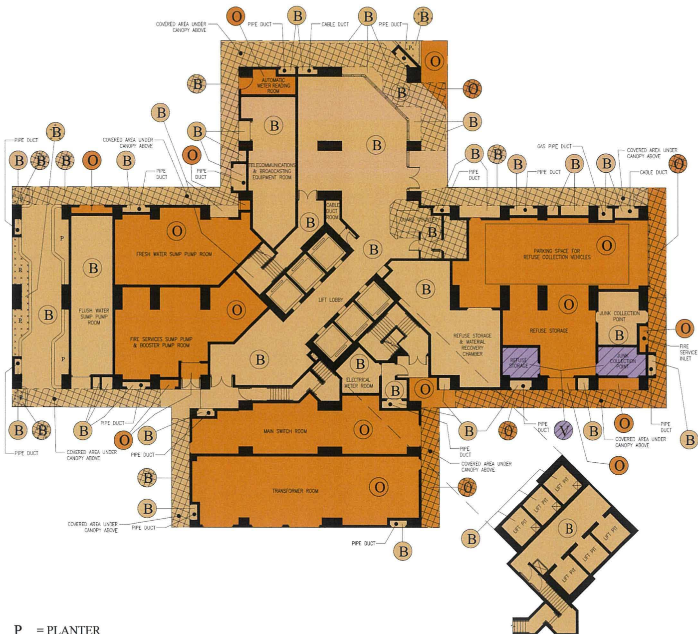
PART PLAN OF LIFT PITS BELOW
