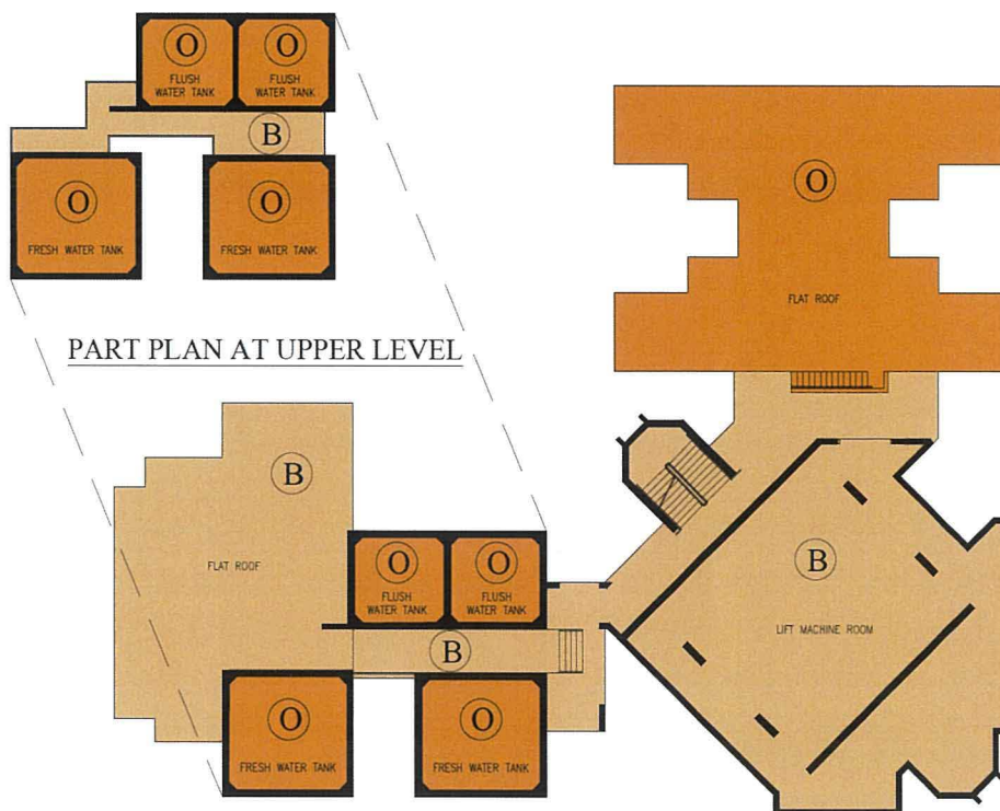
LIFT MACHINE ROOM PLAN
