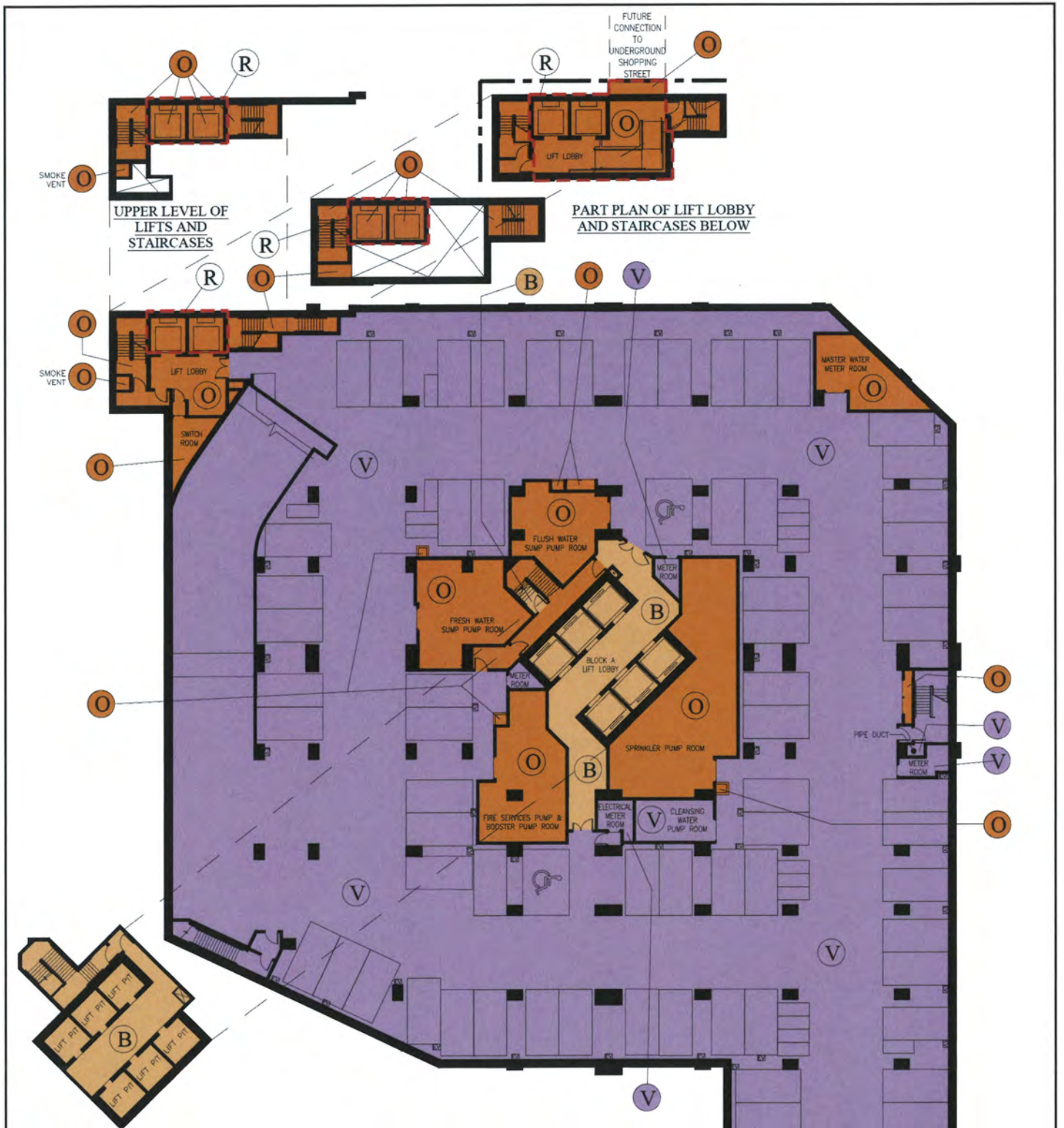
PART PLAN OF LIFT PITS OF BLOCK A BELOW
