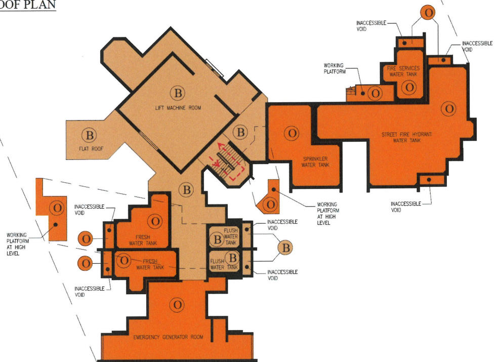
UPPER ROOF PLAN
