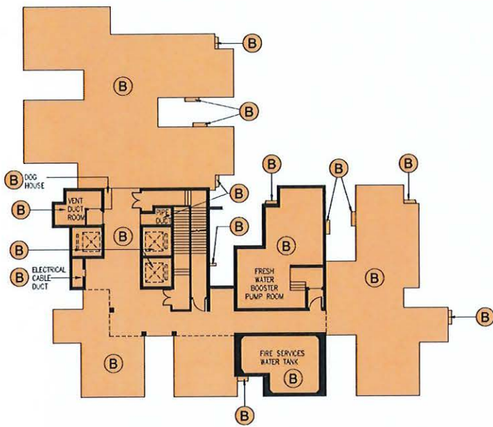
MAIN ROOF PLAN
