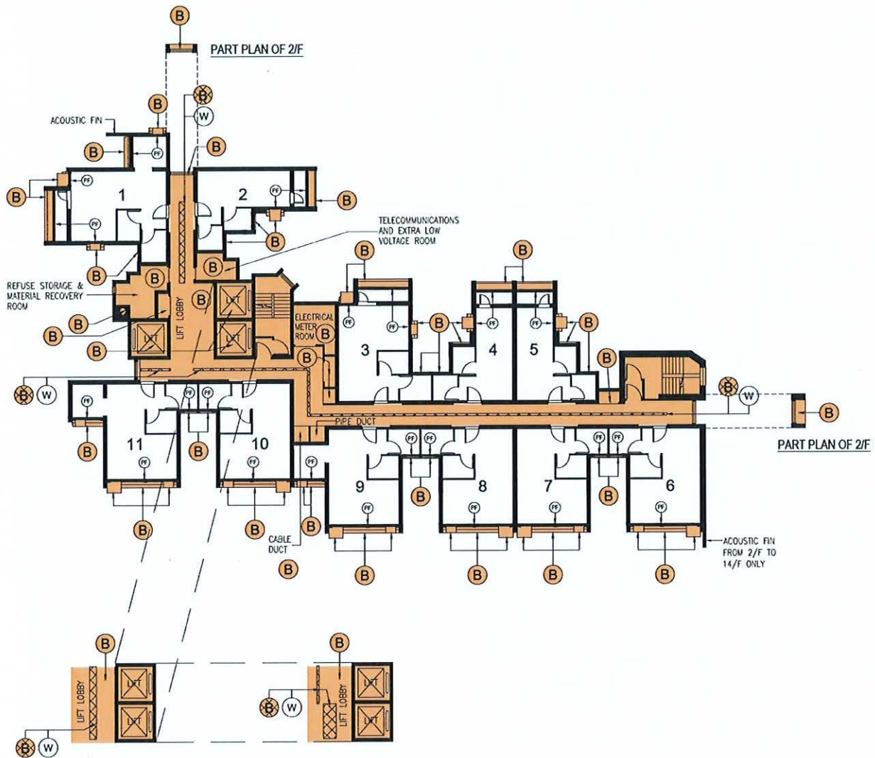
TYPICAL PART PLAN ( 2/F TO 20/F )
