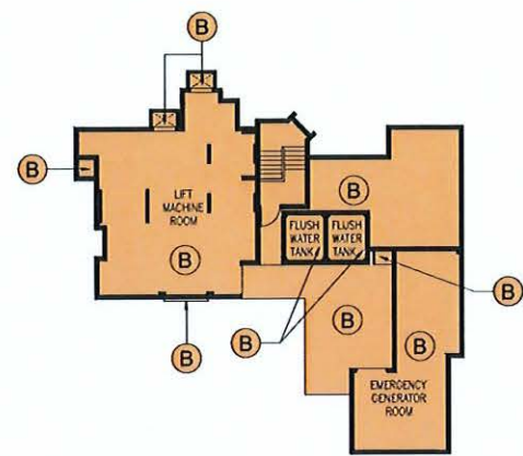
LIFT MACHINE ROOM PLAN
