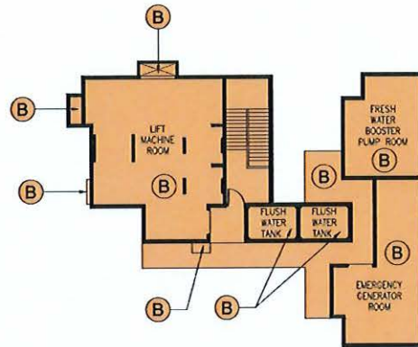
LIFT MACHINE ROOM PLAN
