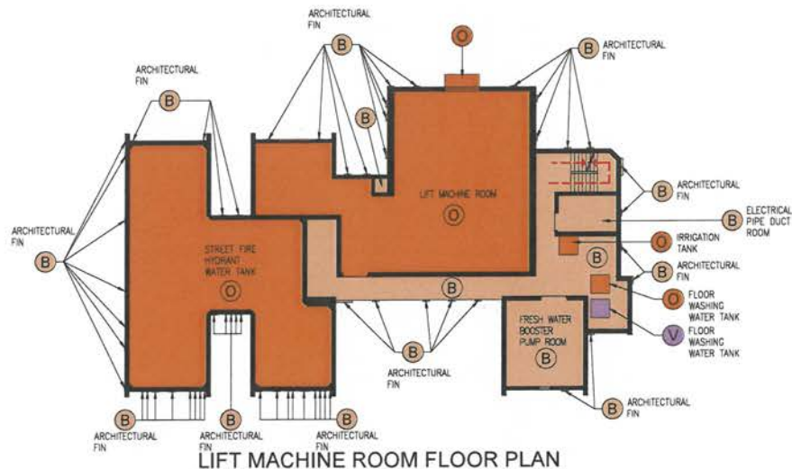
LIFT MACHINE ROOM FLOOR PLAN
