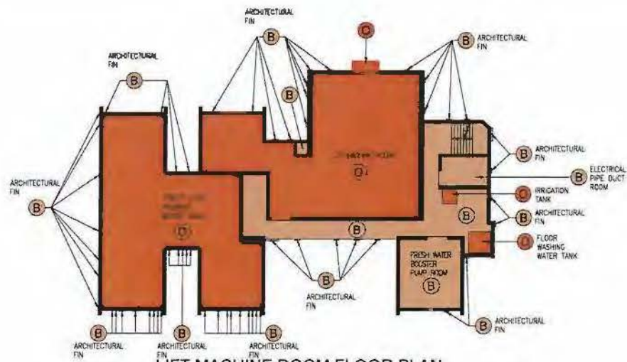
LIFT MACHINE ROOM FLOOR PLAN
