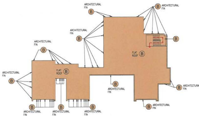
TOP ROOF PLAN
