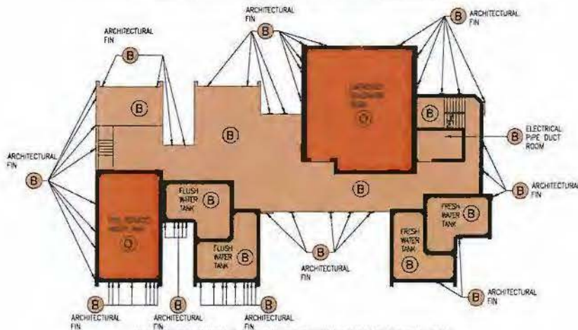
EMERGENCY GENERATOR ROOM PLAN
