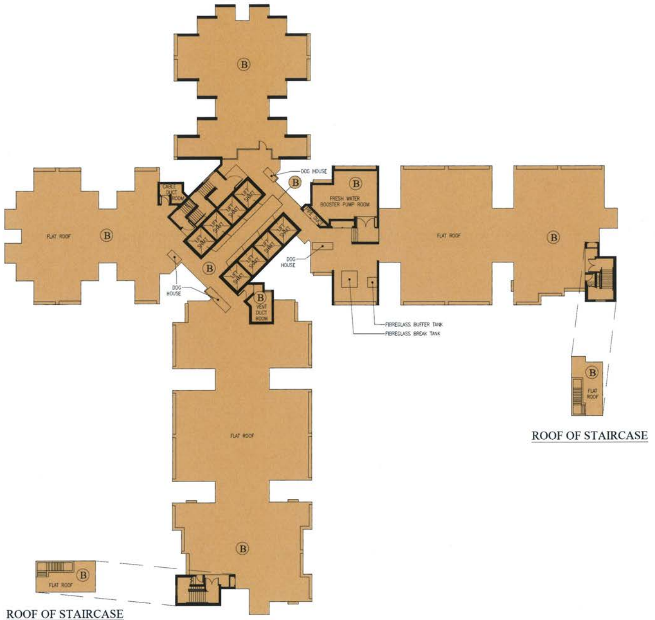
ROOF OF STAIRCASE
