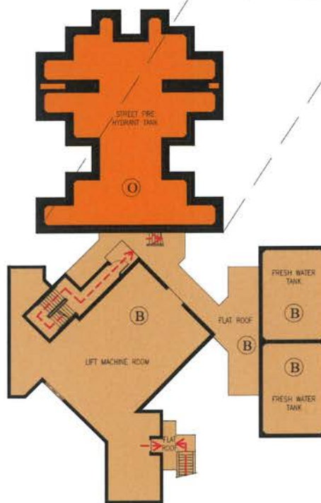
LIFT MACHINE ROOM PLAN
