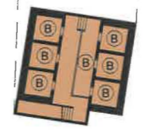
BLOCK B PART PLAN AT LIFT PIT LEVEL
