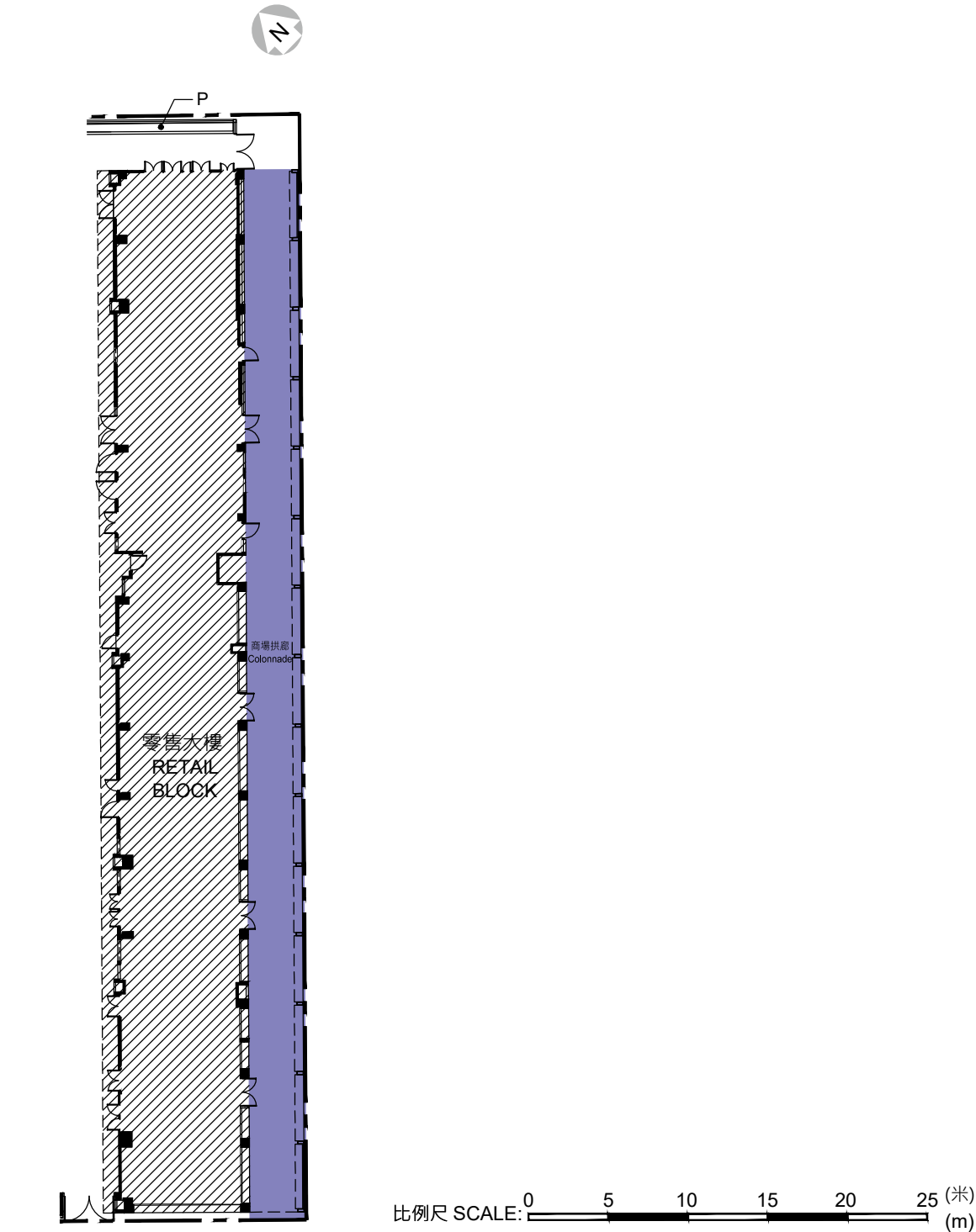
零售大樓地下平面圖 GROUND FLOOR PLAN OF RETAIL BLOCK
