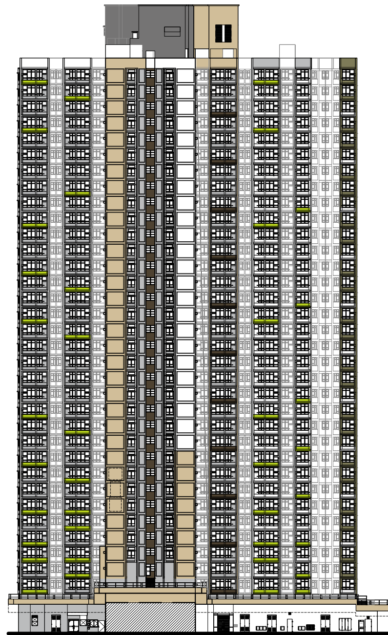
西南面立面圖 “1” South West Elevation Plan “1”
