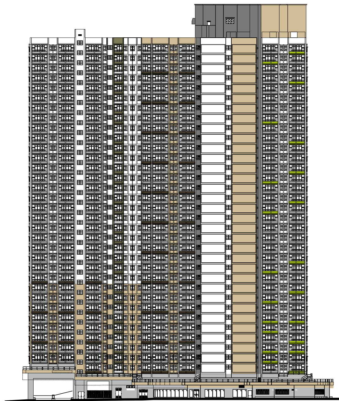
東南面立面圖 "2" South East Elevation Plan "2"
