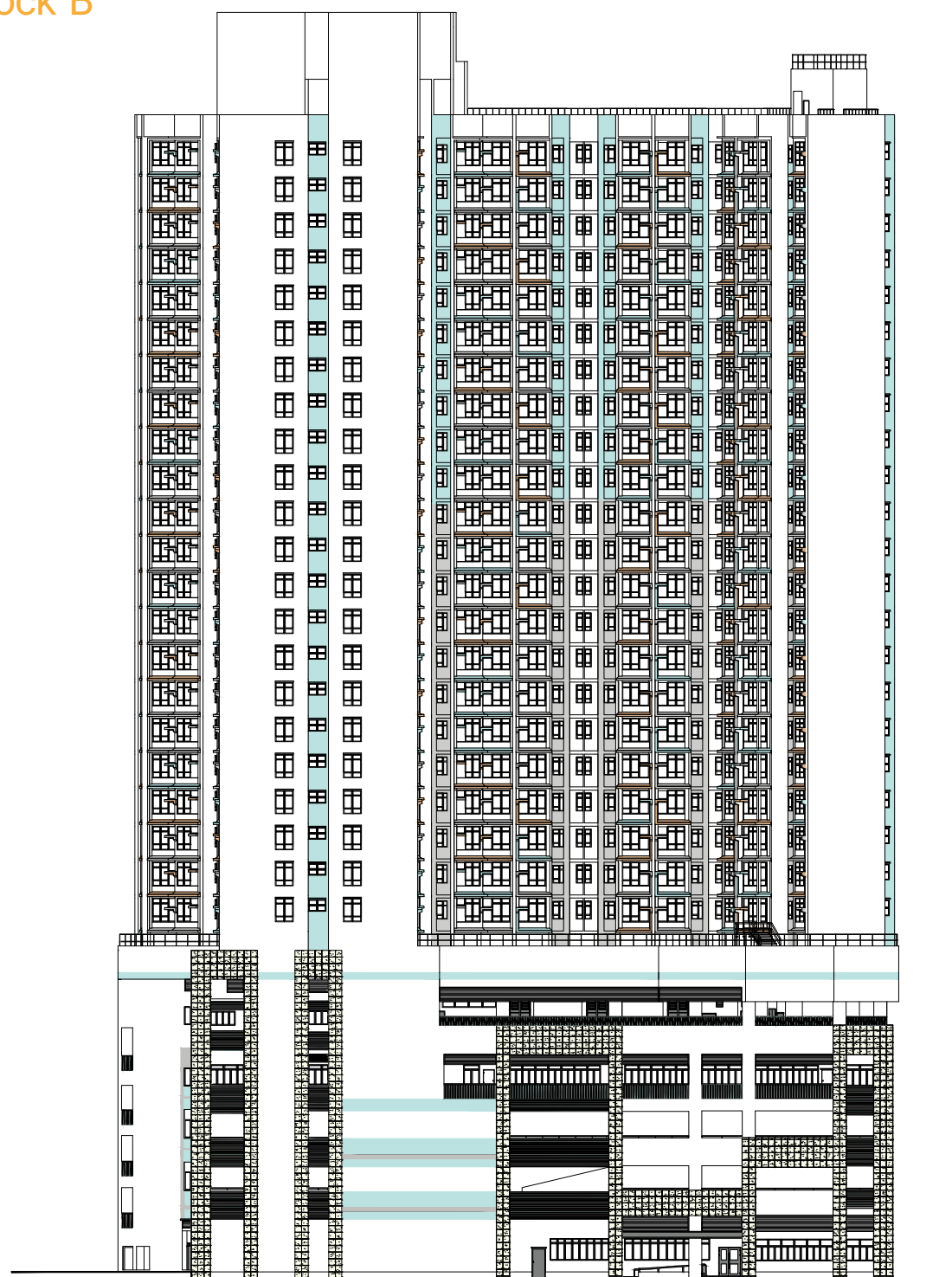
東南面立面圖 "1" South East Elevation Plan "1"
