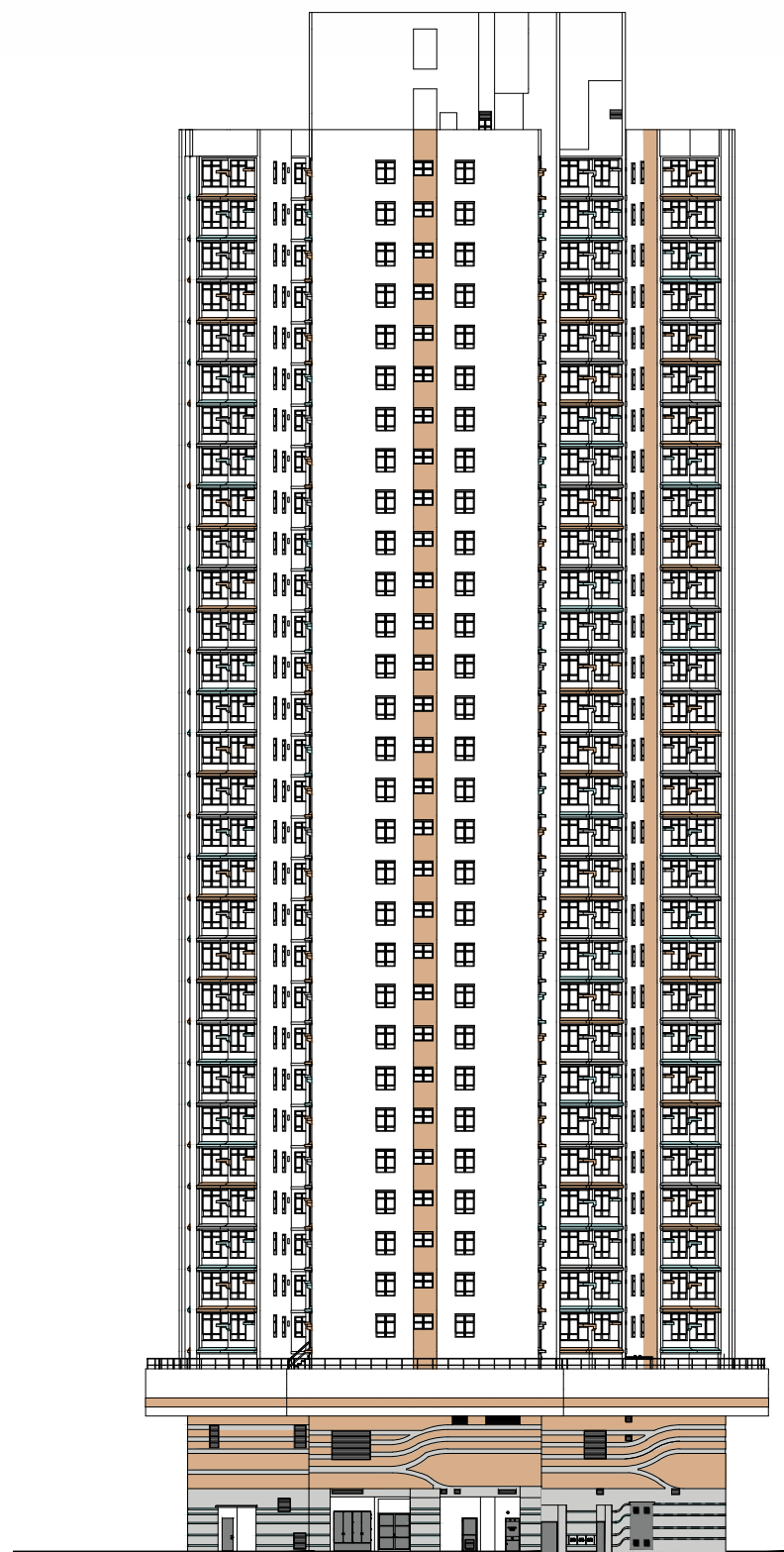
東南面立面圖“1” South East Elevation Plan “1”
