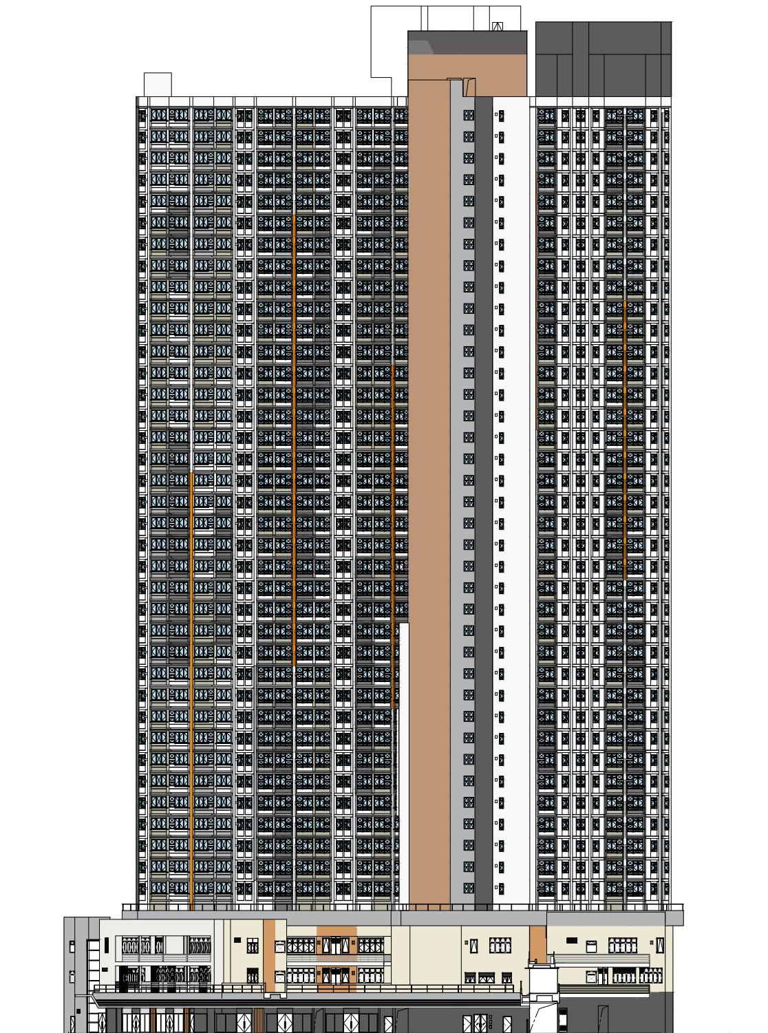
西南面立面圖 "4" South West Elevation Plan "4"
