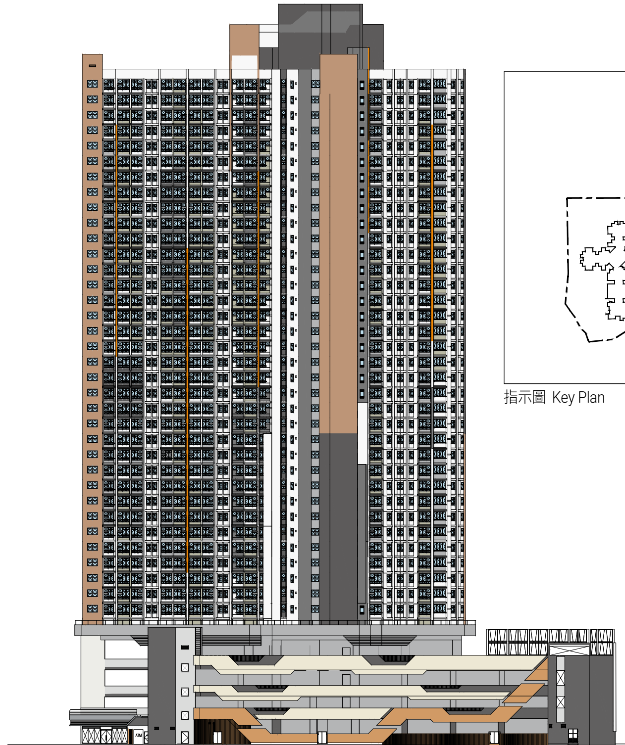
西北面立面圖 "1" North West Elevation Plan "1"
