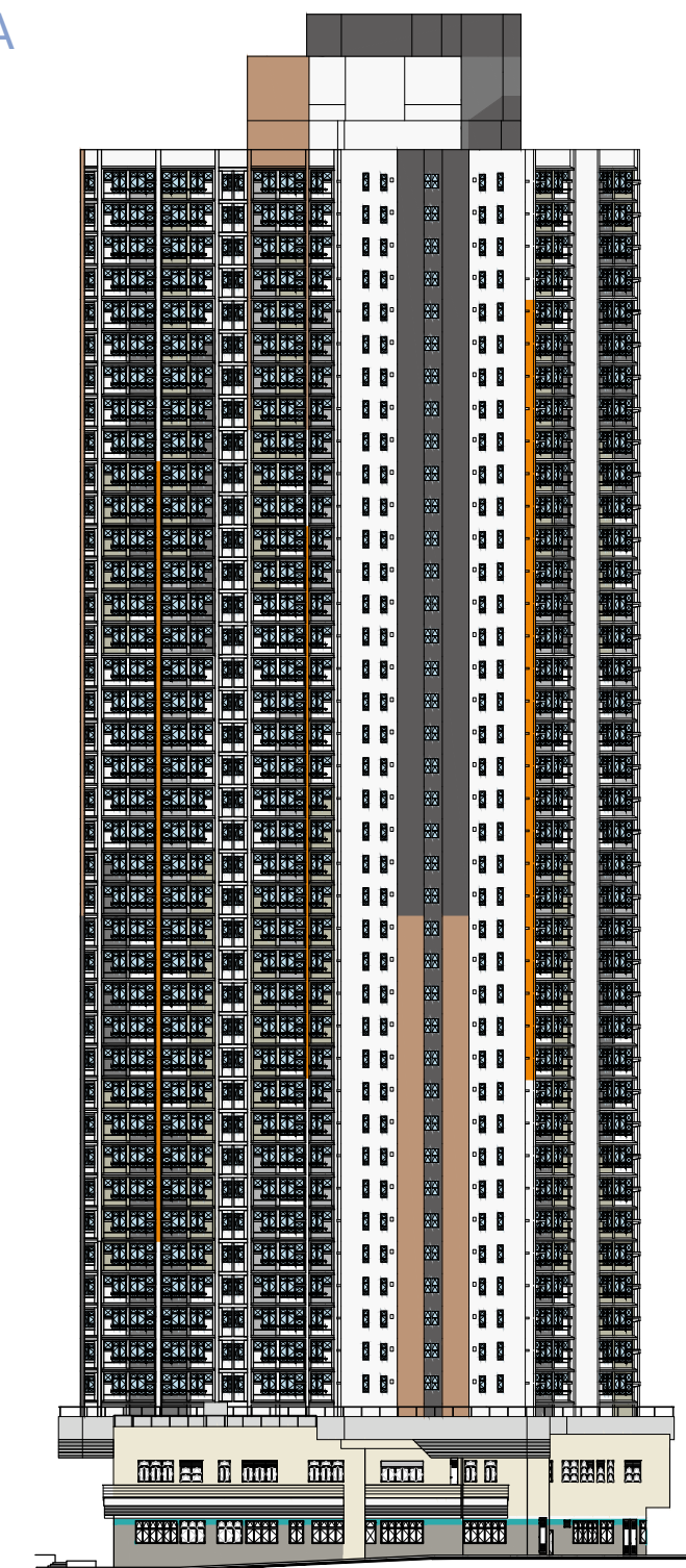
東南面立面圖 "3" South East Elevation Plan "3"
