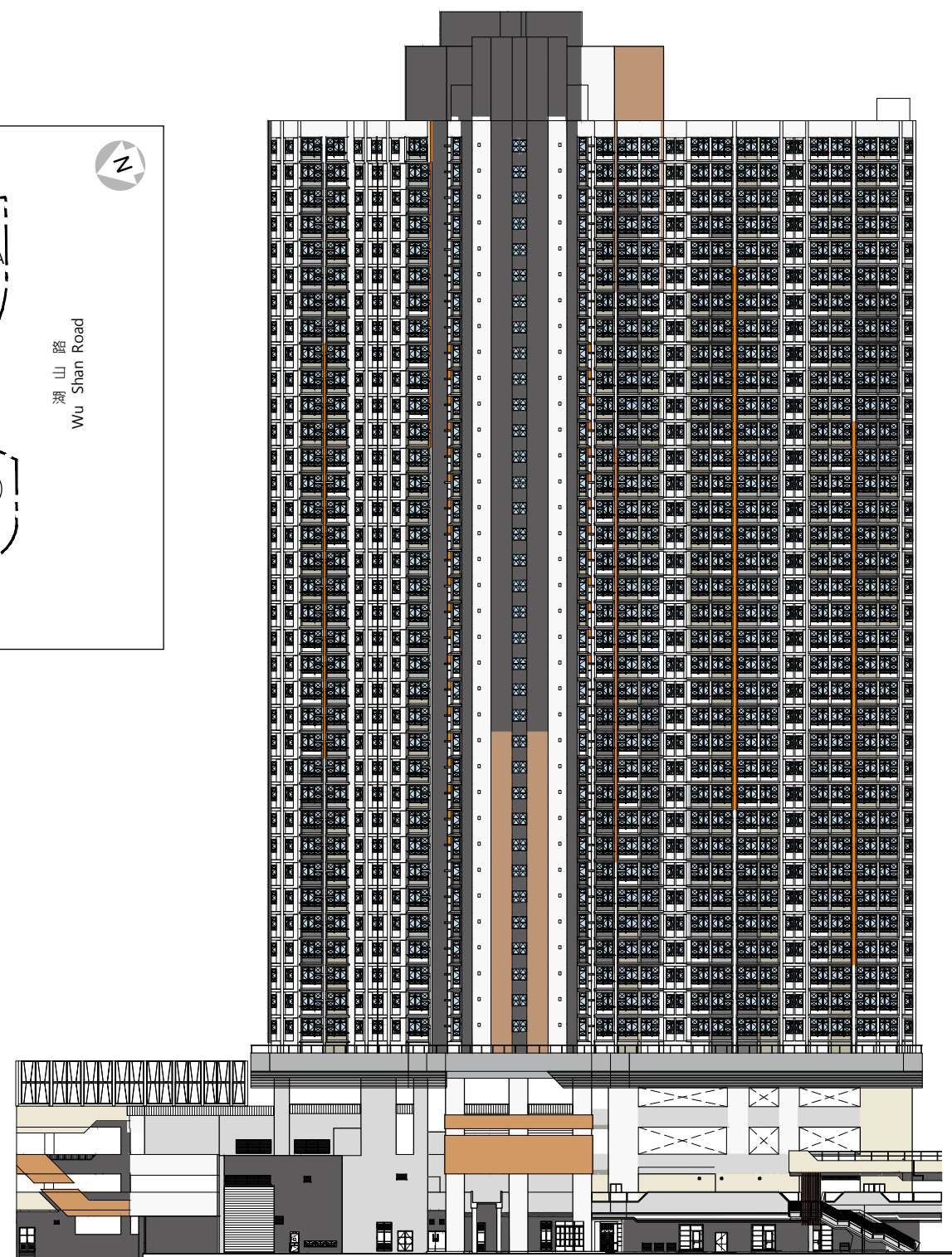
東南面立面圖 "3" South East Elevation Plan "3"
