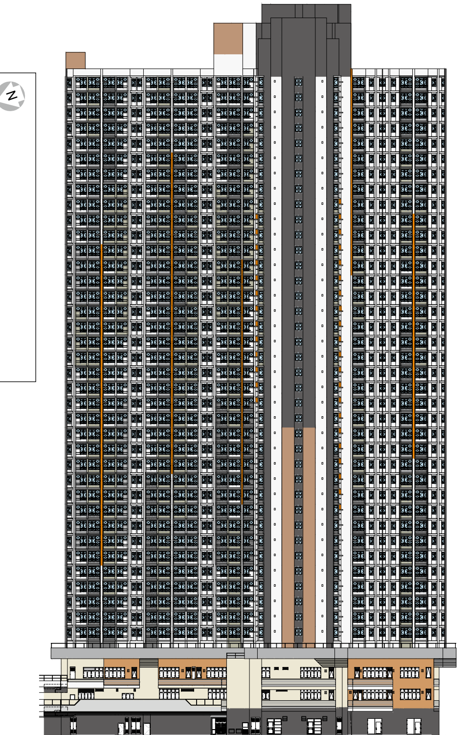
東南面立面圖 "3" South East Elevation Plan "3"
