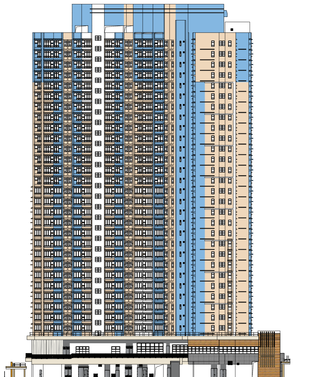
西南面立面圖 "3" South West Elevation Plan "3"
