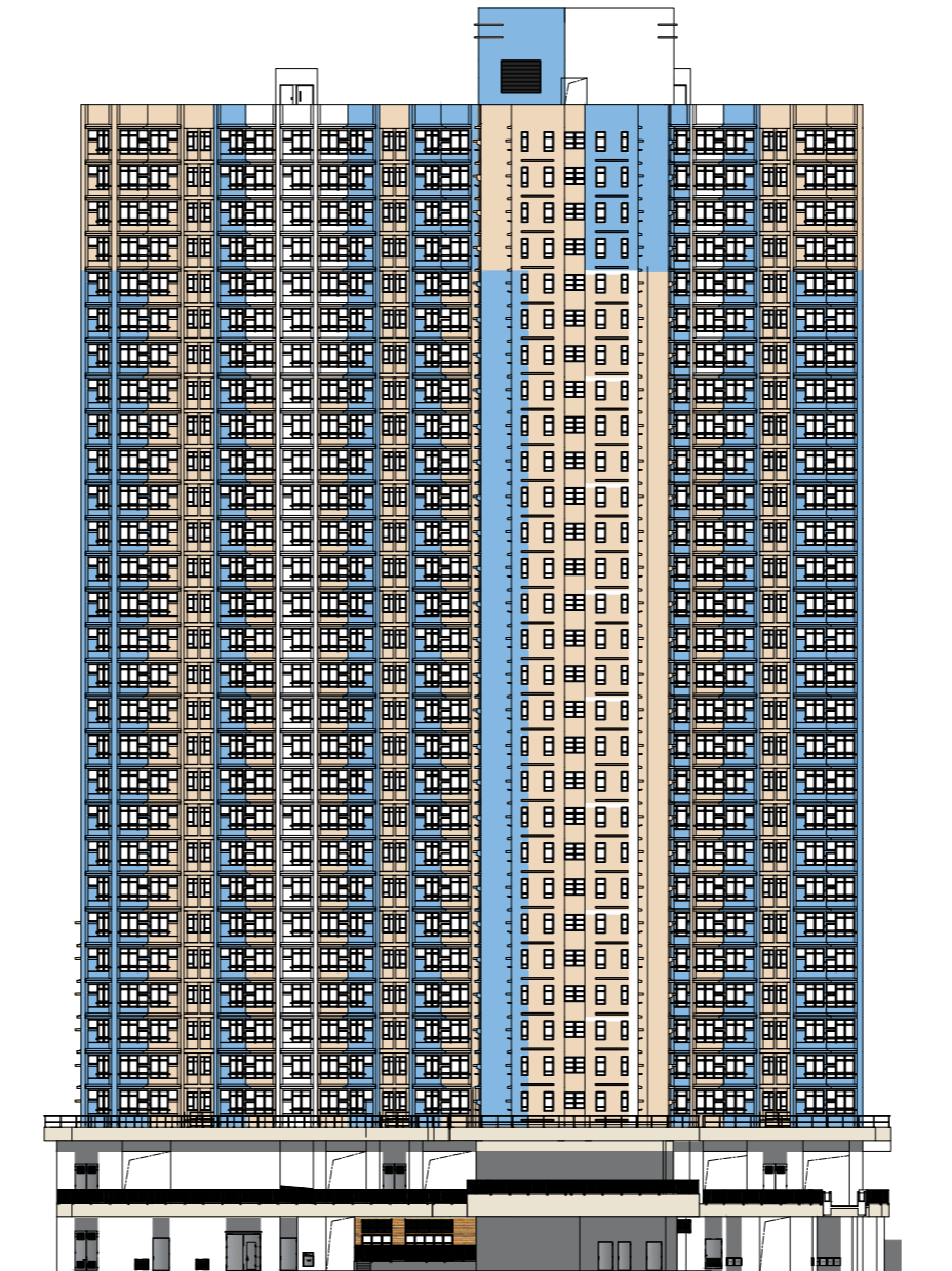
西北面立面圖 "4" North West Elevation Plan "4"
