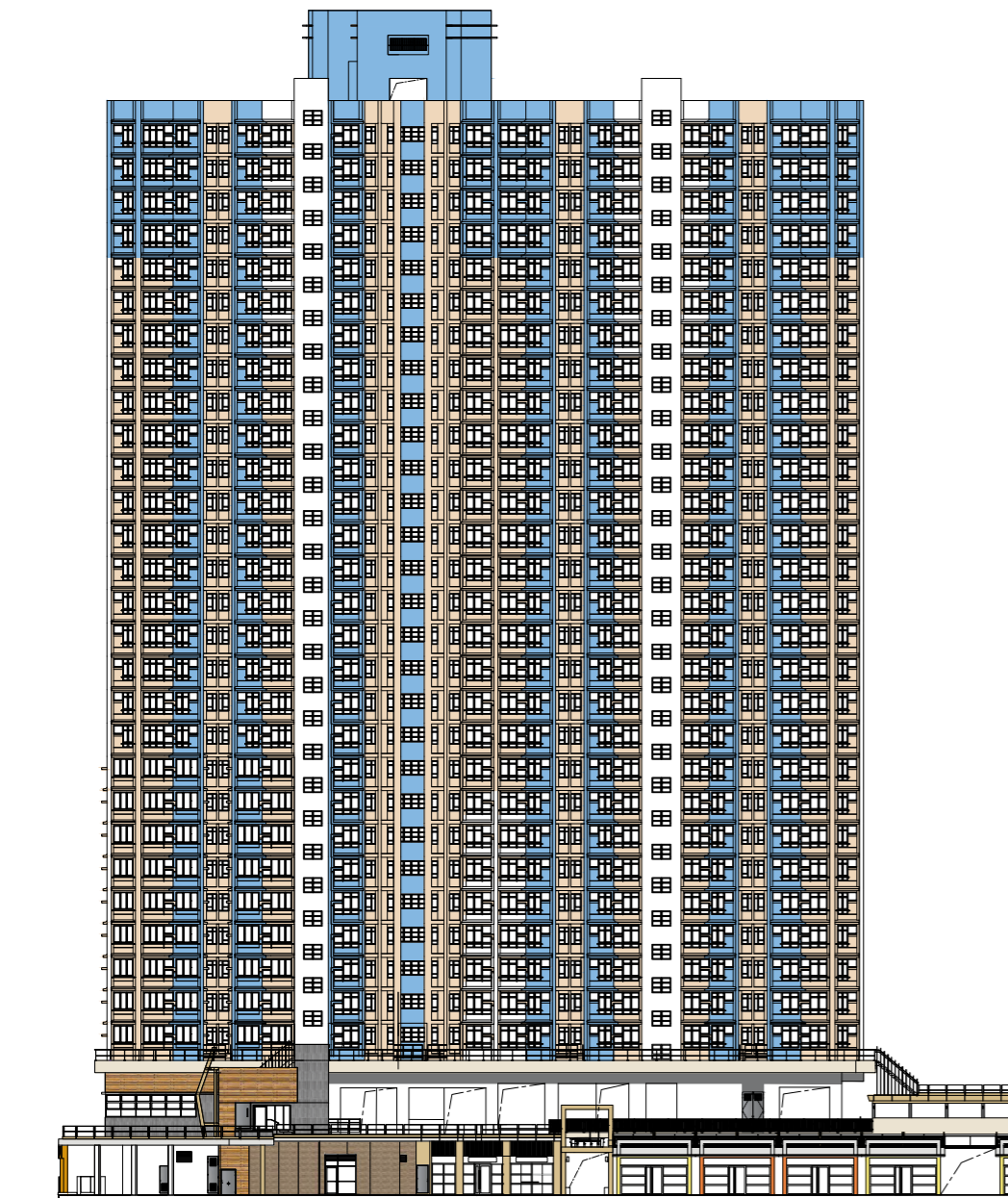
東南面立面圖 "1" South East Elevation Plan "1"
