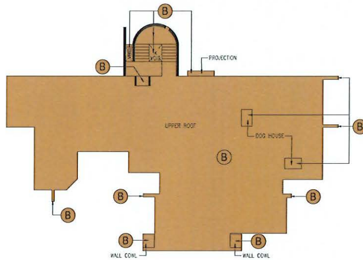
UPPER ROOF SECOND FLOOR PLAN
