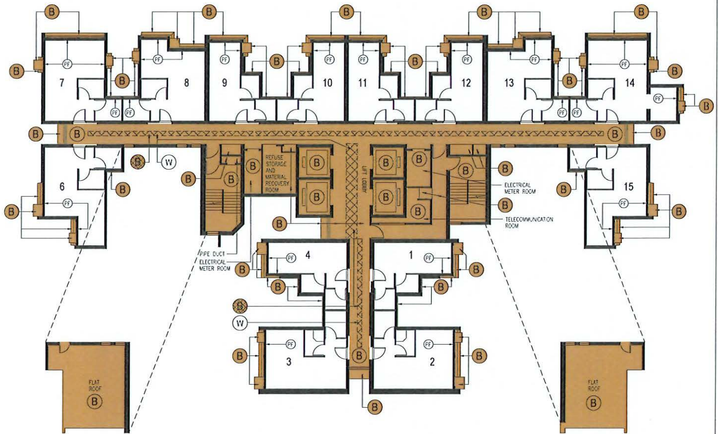
PART PLAN AT 35/F ONLY
