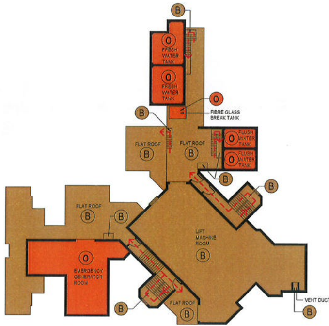
UPPER ROOF PLAN
