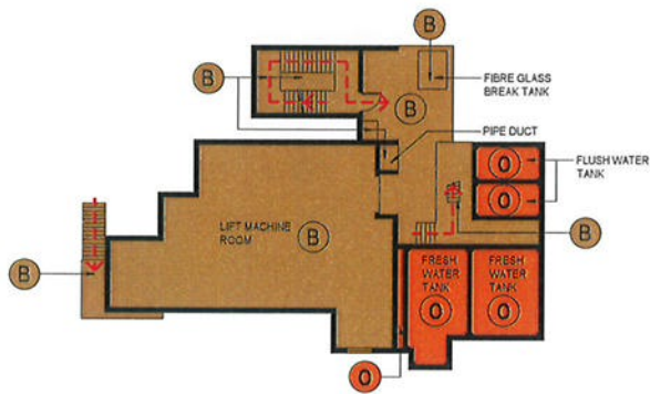
LIFT MACHINE ROOM FLOOR PLAN
