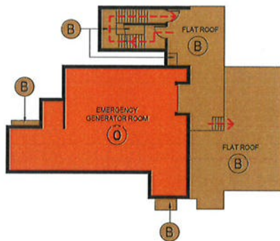
UPPER ROOF PLAN
