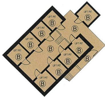
BLOCK C PART PLAN AT LIFT PIT LEVEL
