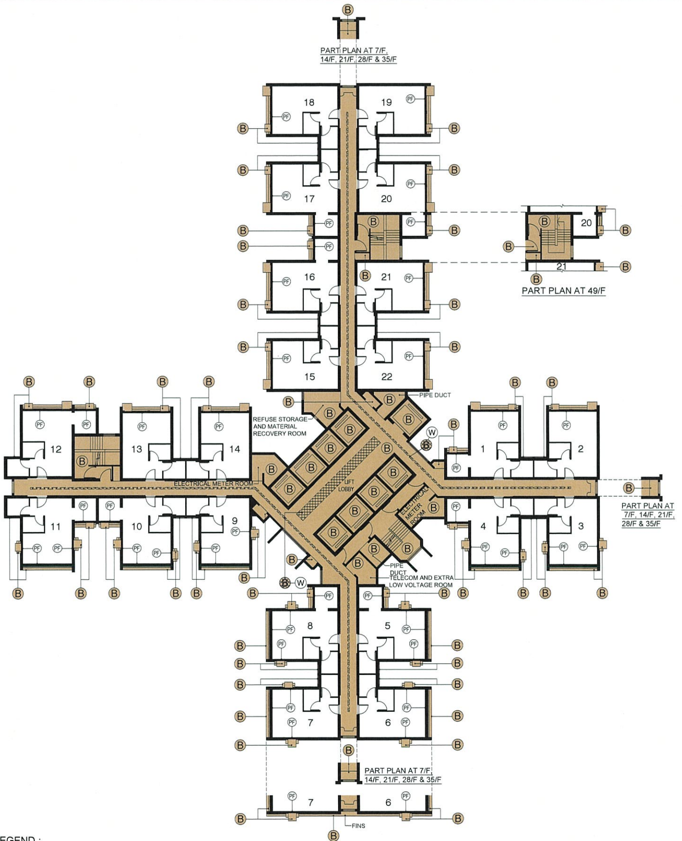
2/F PART PLAN
