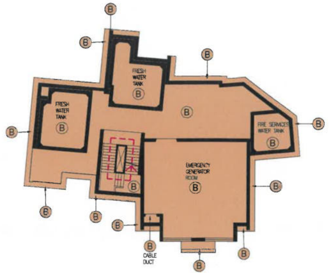
WATER TANK LEVEL PLAN
