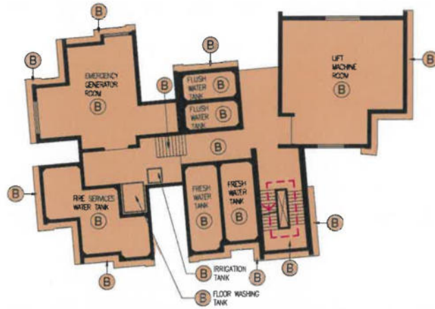
LIFT MACHINE ROOM FLOOR PLAN
