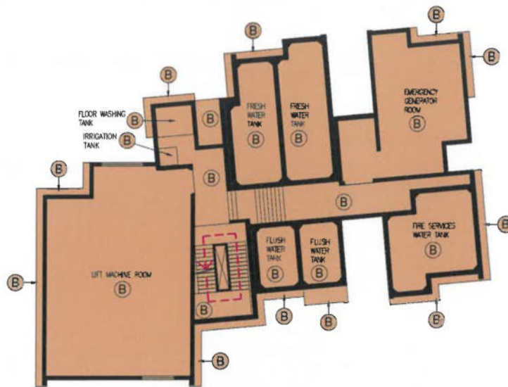
LIFT MACHINE ROOM FLOOR PLAN
