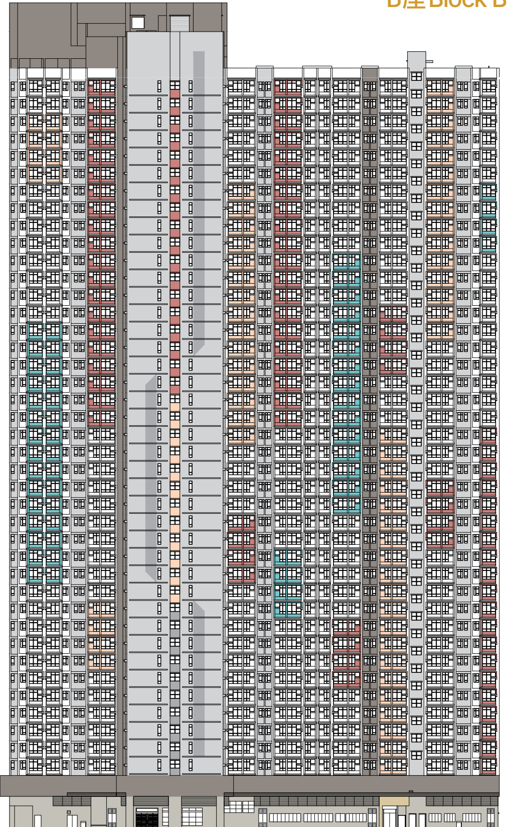
西南面立面圖"3" South West Elevation Plan "3"
