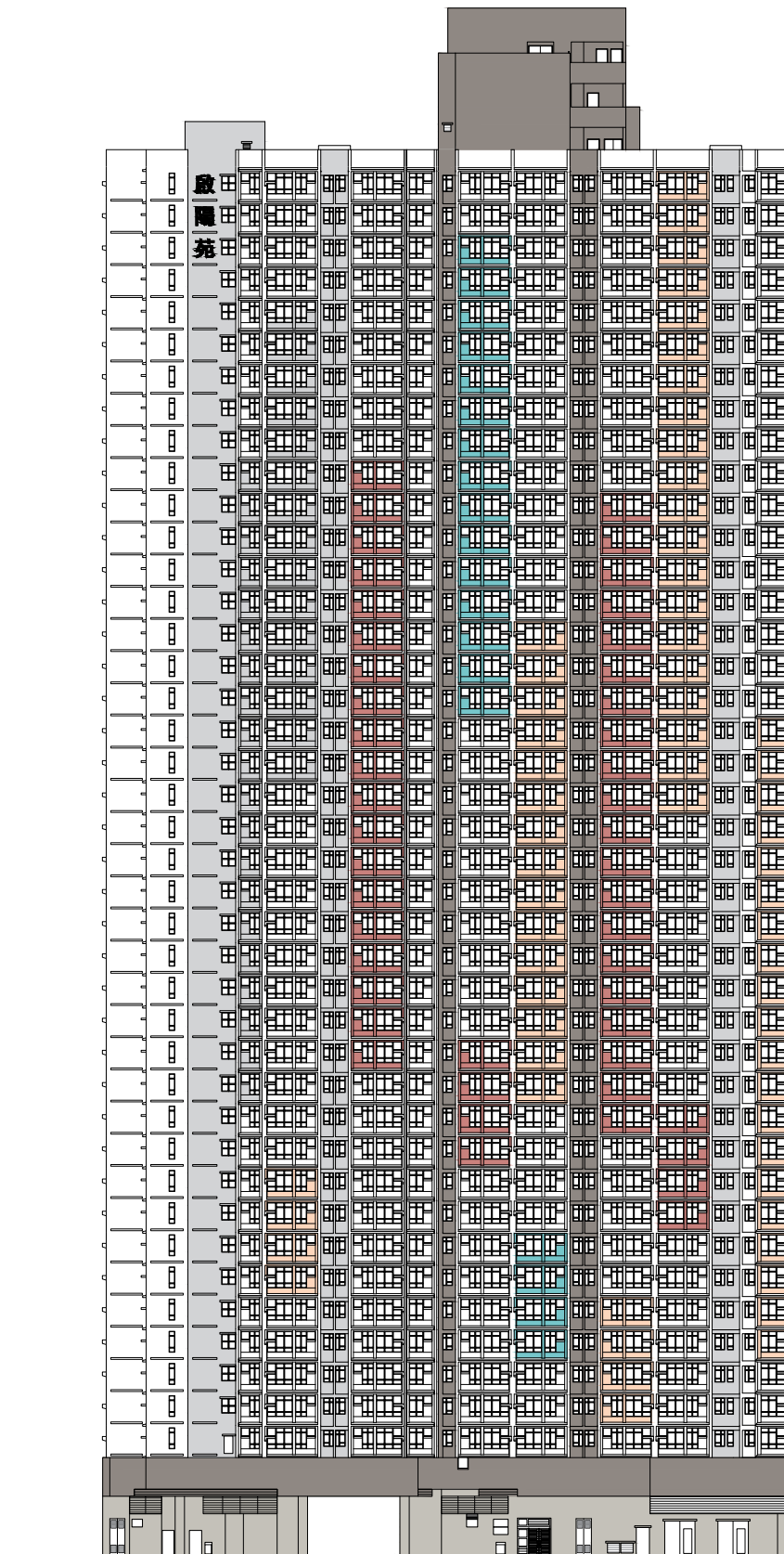
西北面立面圖"4" North West Elevation Plan "4"
