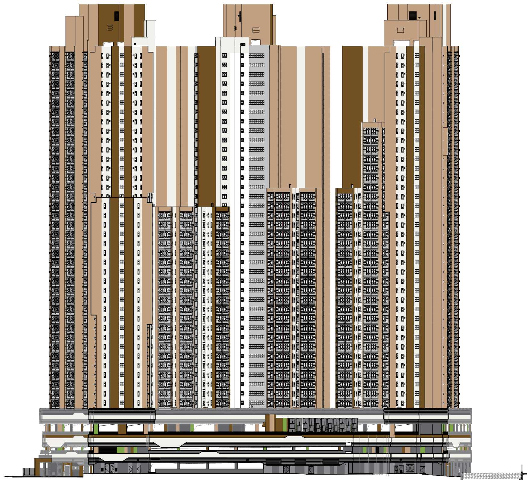
南面立面圖 "3" South Elevation Plan "3"
