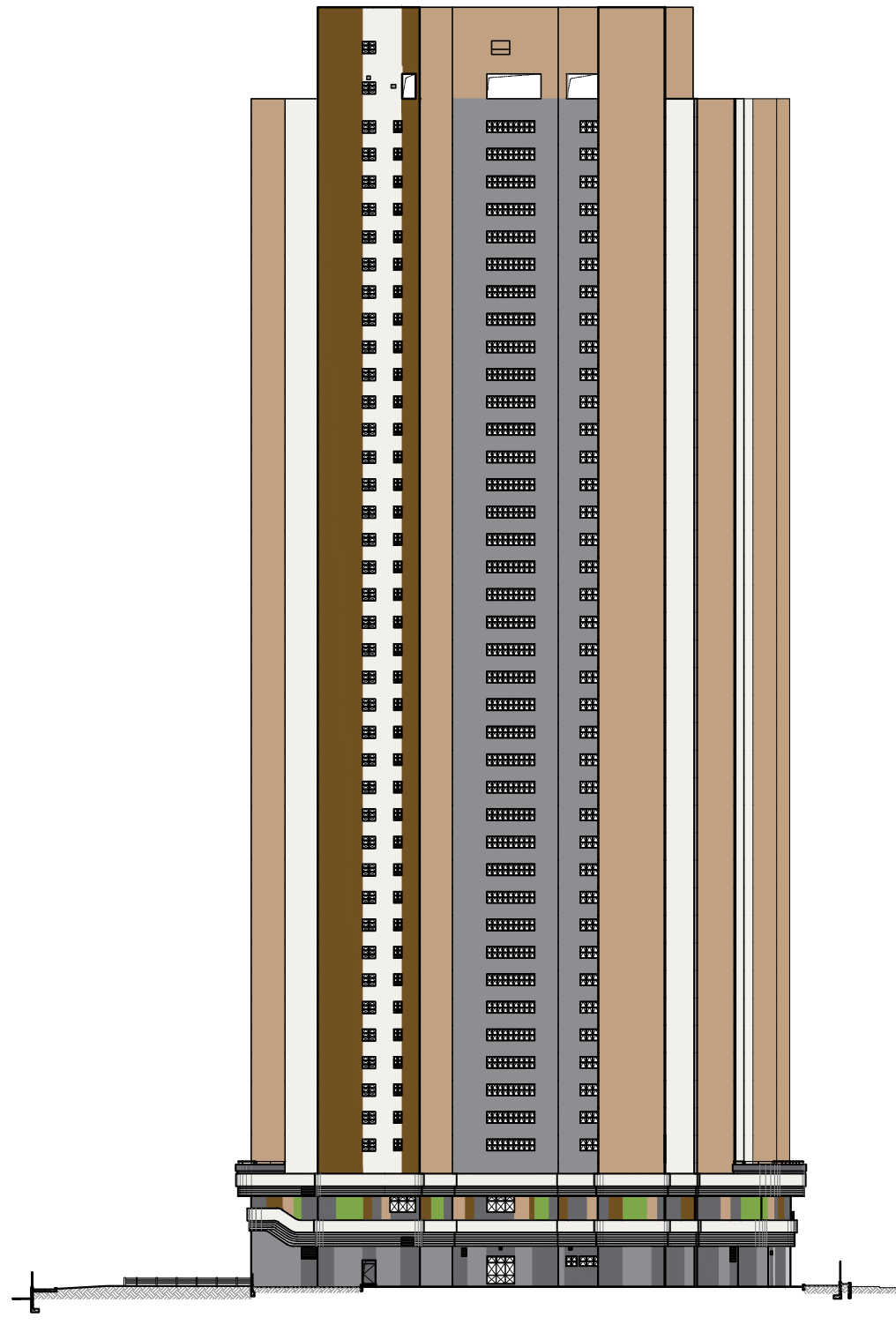
西南面立面圖 "4" South West Elevation Plan "4"
