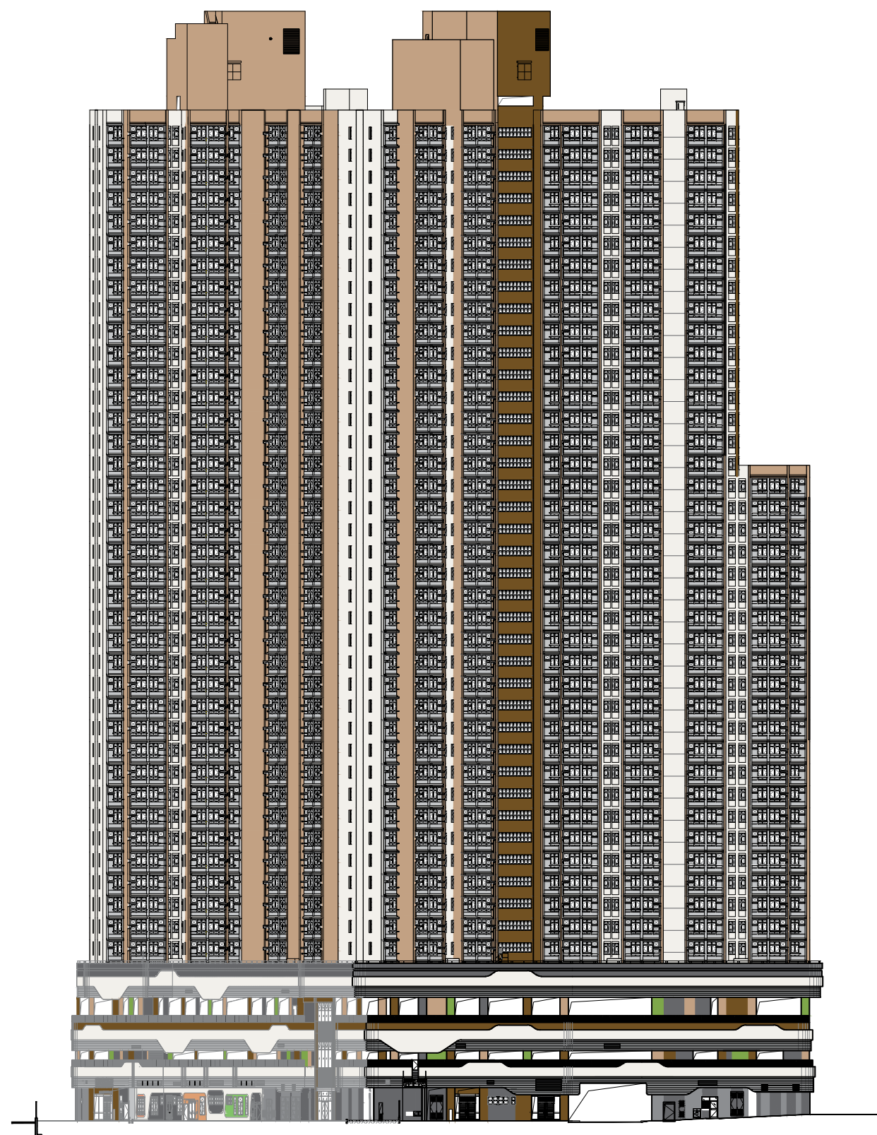
西面立面圖"4" West Elevation Plan "4"
