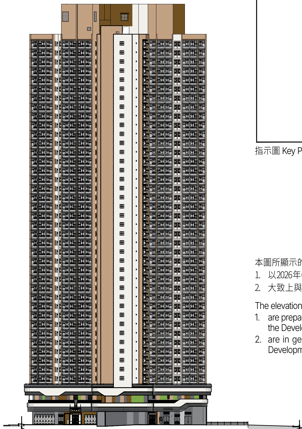
東南面立面圖 "2" South East Elevation Plan "2"
