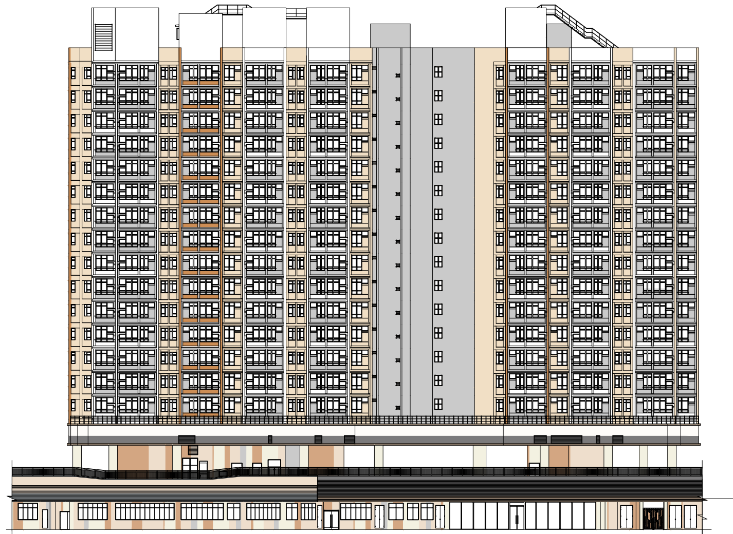
東北面立面圖 "1" North East Elevation Plan "1"
