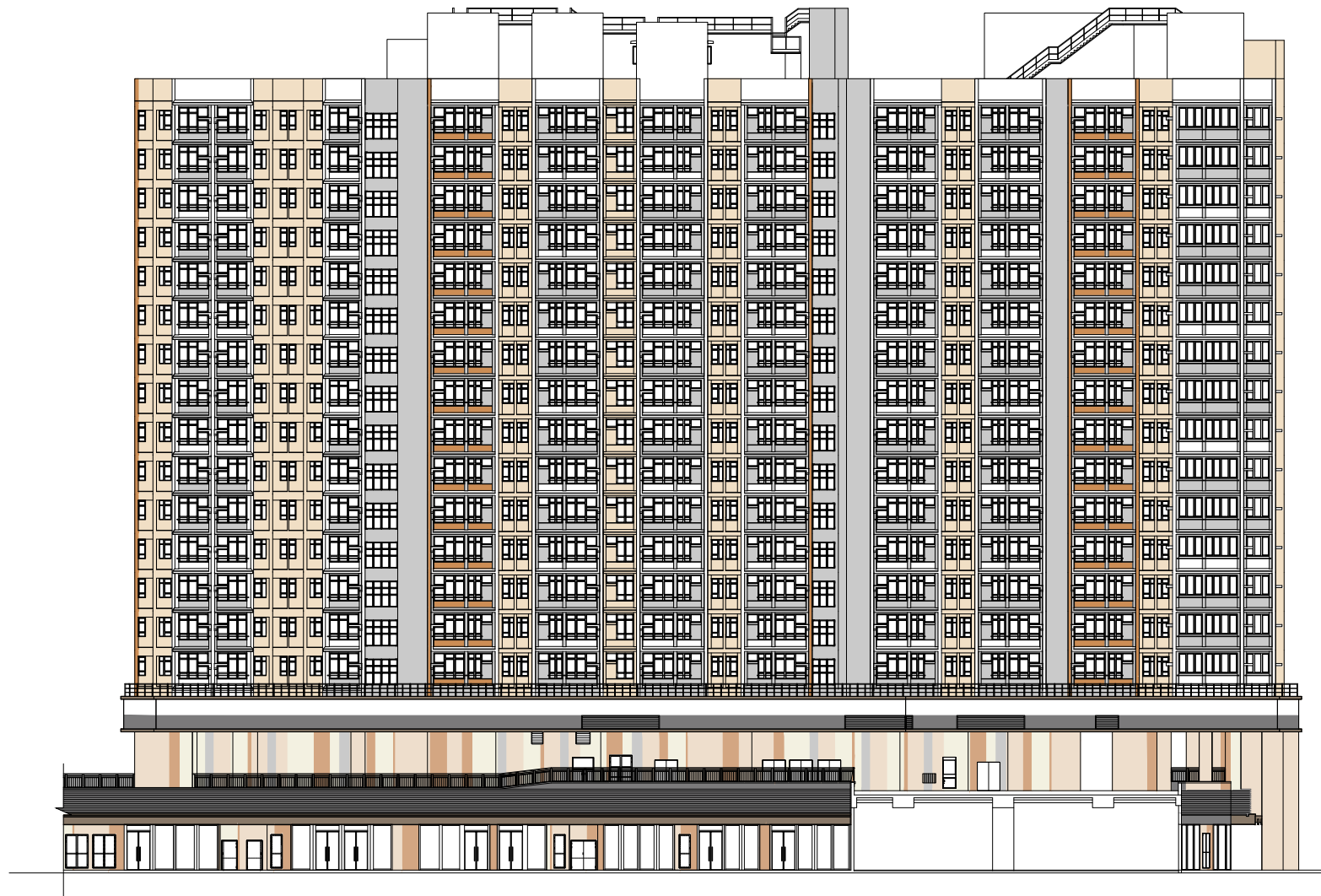
東北面立面圖"3" North East Elevation Plan "3"
