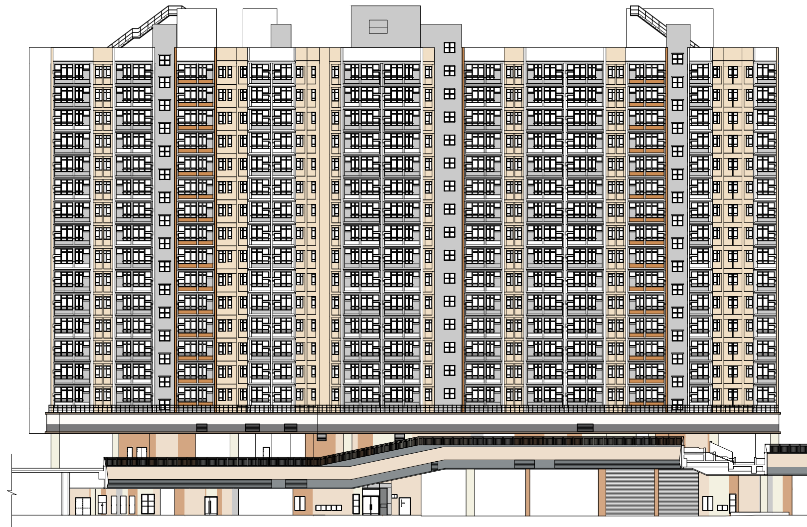
西北面立面圖 "3" North West Elevation Plan "3"
