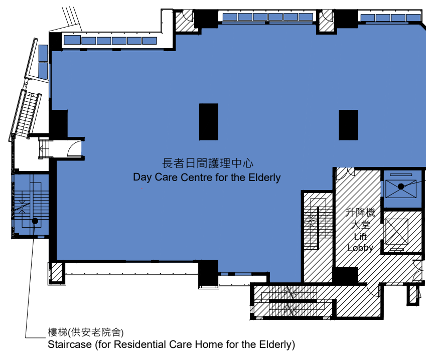
地下長者日間護理中心部分平面圖 GROUND FLOOR PART PLAN OF DAY CARE CENTRE FOR THE ELDERLY
