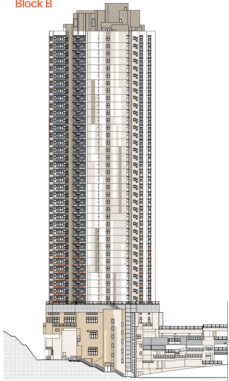
南面立面圖 "2" South Elevation Plan "2"
