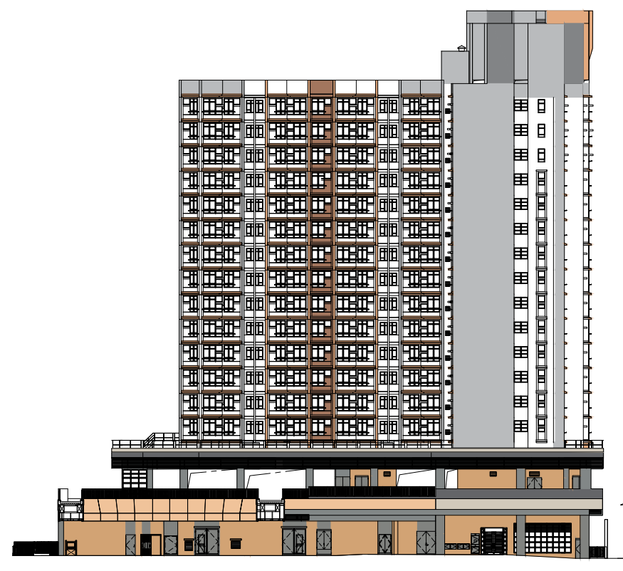
西南面立面圖"3" South West Elevation Plan "3"
