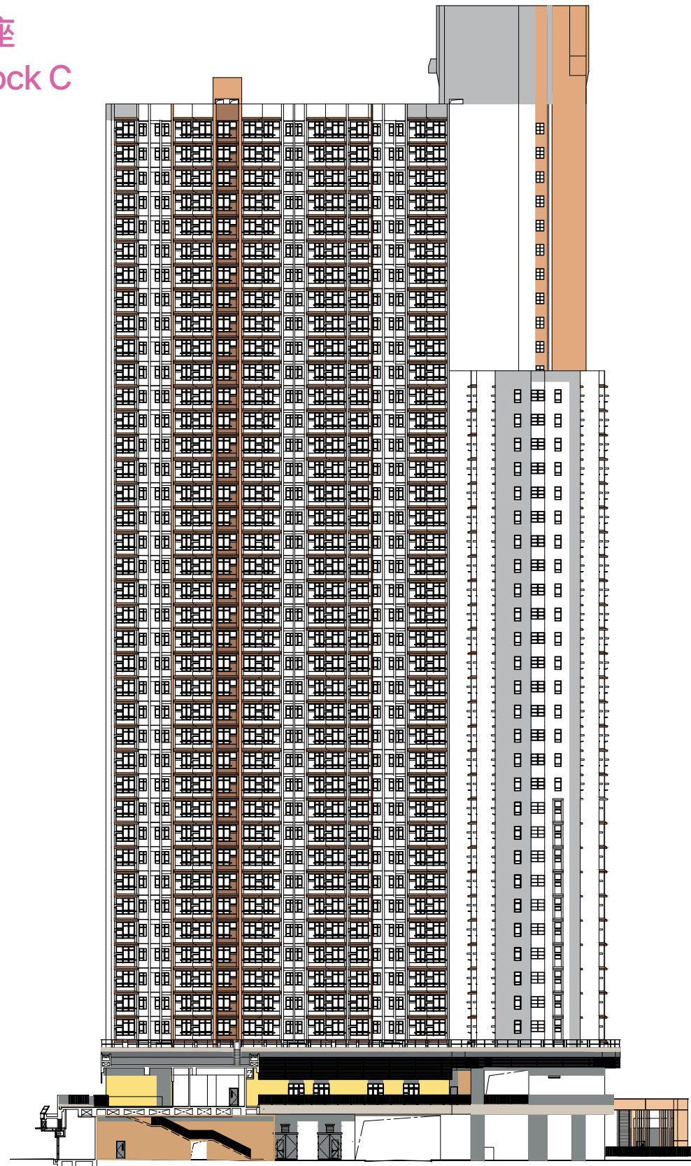
西南面立面圖 "3" South West Elevation Plan "3"
