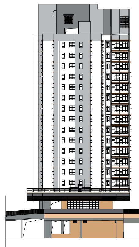
西北面立面圖"2" North West Elevation Plan "2"
