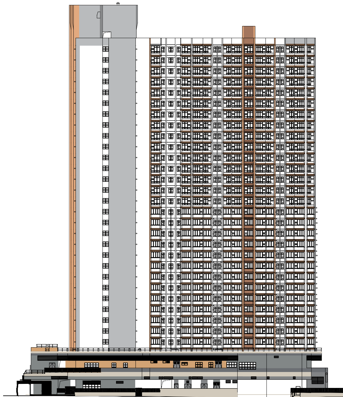
西南面立面圖"1" South West Elevation Plan "1"
