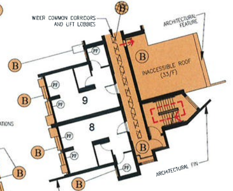
PART PLAN AT 33/F-40/F
