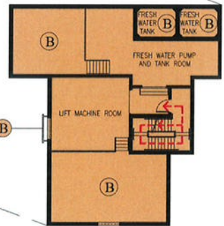
LIFT MACHINE ROOM PLAN
