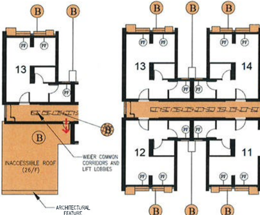
PART PLAN AT 26/F-32/F
