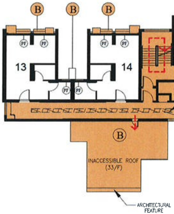
PART PLAN AT 33/F-40/F
